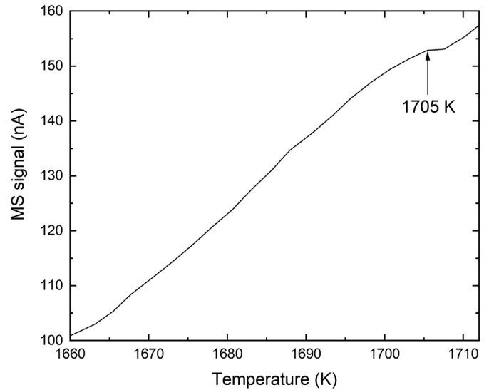
Fig. 6. Detection of \text{PuF}_3 melting point by KEMS. The signal shows a marked change of slope.
