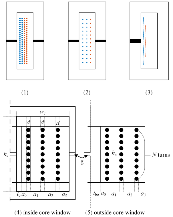
Fig. 7. Illustration of winding configurations, (1) and (2) equal layer winding heights with different \Delta_{hei} and \Delta_{wid} , (3) different layer winding heights. Notation of windings inside the core window (4) and outside the core window (5).
