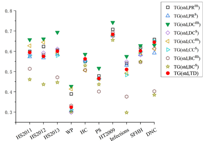
Fig. 8. Kendall correlation coefficient \tau between the node centrality score obtained from R_{norm} and temporal gravity models for 10 empirical networks.
