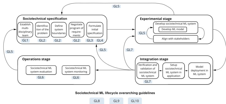
Fig. 4 Visualisation of the sociotechnical ML lifecycle with the developed guidelines. The larger boxes are the different stages of the ML lifecycle. Within each stage, the smaller boxes denote activities. The blue-colored boxed numbered GL1-GL10 denote the activities and points in the lifecycle where the guidelines apply
