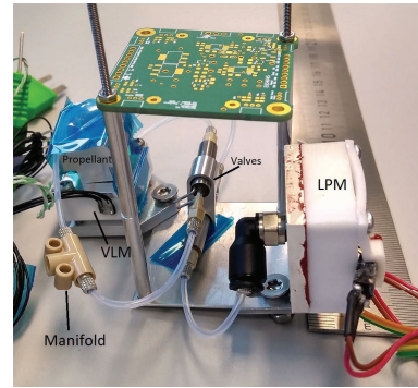
Fig. 3. Assembly of the prototype completed in the cleanroom; pressure sensors and wiring are not attached.
