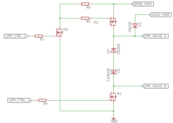
Fig. 10. Valve control circuitry.
