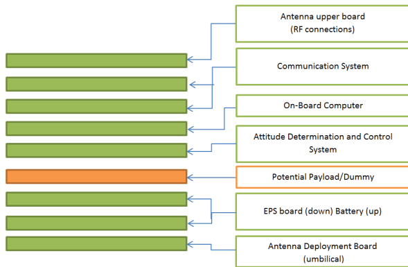
Fig. 2. Delfi-PQ subsystems.
