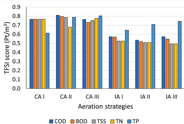
Fig. 5. TFSI scores for each aeration strategy with respect to each pollutant considered.
