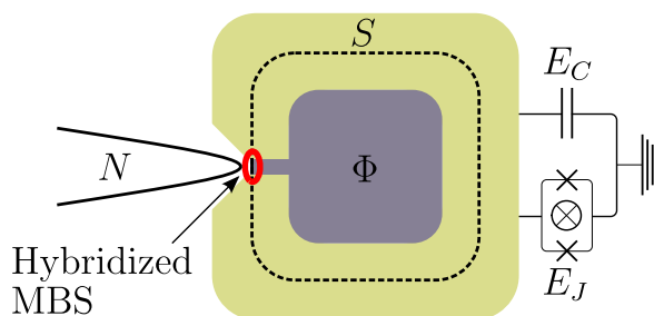
FIG. 1. Setup consists of a QSHE insulator (dark gray) with its edge (dashed line) partially covered by a superconducting ring. The proximity-induced gap in the QSHE edge forms two hybridized MBS at the part of the edge not covered by the superconductor. A tunable Josephson junction couples the superconducting ring to the superconducting lead. Finally, the normal lead weakly couples to the quantum spin Hall edge in the junction region.
