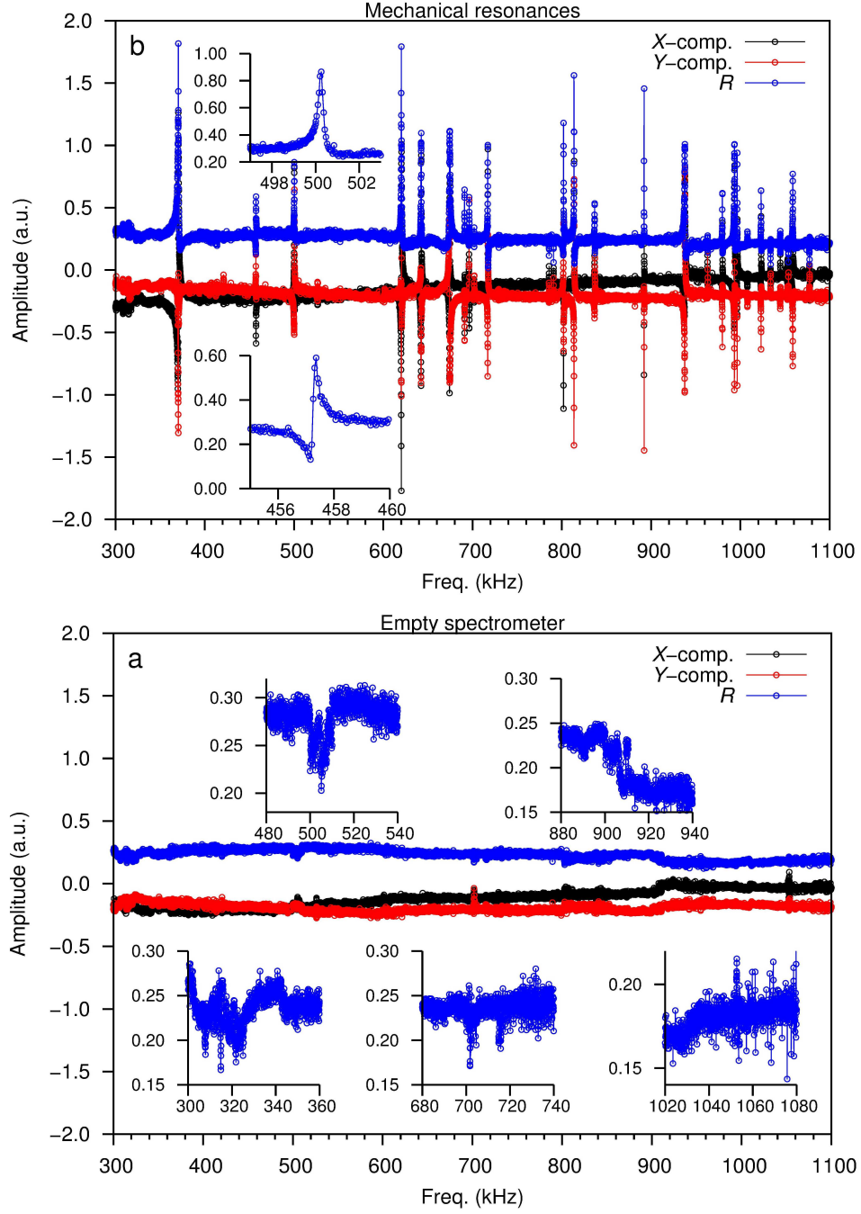
Figure 3: The X -, Y -, components and the magnitude signal R (see text) of the background spectrum measured on an empty spectrometer (a) and for the rectangular parallelepiped sample used in this study (b). Inset shows: (a) the maximum frequency disturbances caused by the setup (see text), (b) typical resonant lines. A line between the experimental points is given as a guide to the eye.
