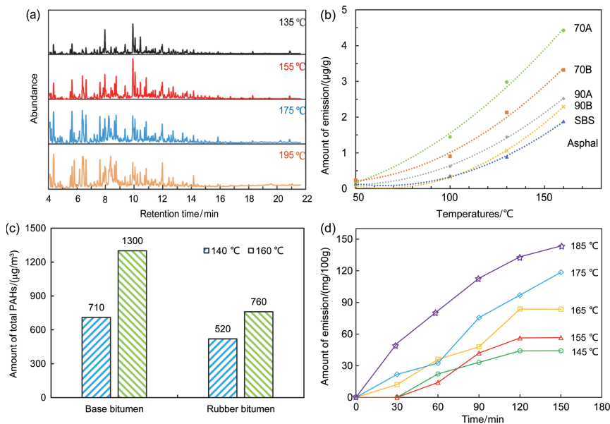
图 16 沥青 VOCs 的温度释放特性 [10,19,58,60] Fig. 16 Release characteristics with temperature of asphalt VOCs [10,19,58,60]
