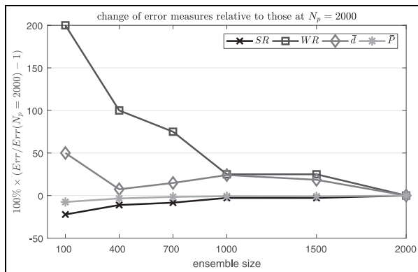
Figure 16. The influence of N_p on the data assimilation results (states are retrieved through interpolation; \sigma_e = 3.0, \sigma_t = 3.0 ); the performance indicators are relative to those at N_p = 2000 .
