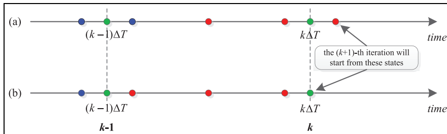
Figure 4. The state points generation process (the blue (generated in the (k - 1) -th iteration) and red (generated in the k -th iteration) dots represent state points in a discrete event state process, while the green dots represent interpolated state points; color online only).
