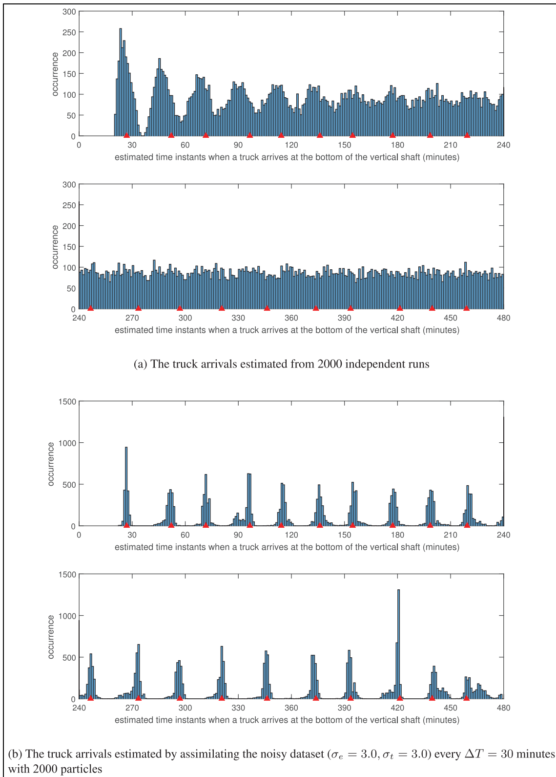
Figure 10. A general view of the estimation results of truck arrivals at the bottom of the vertical shaft with and without assimilating noisy data (each red triangle represents a truck arrival in ground truth; color online only).
