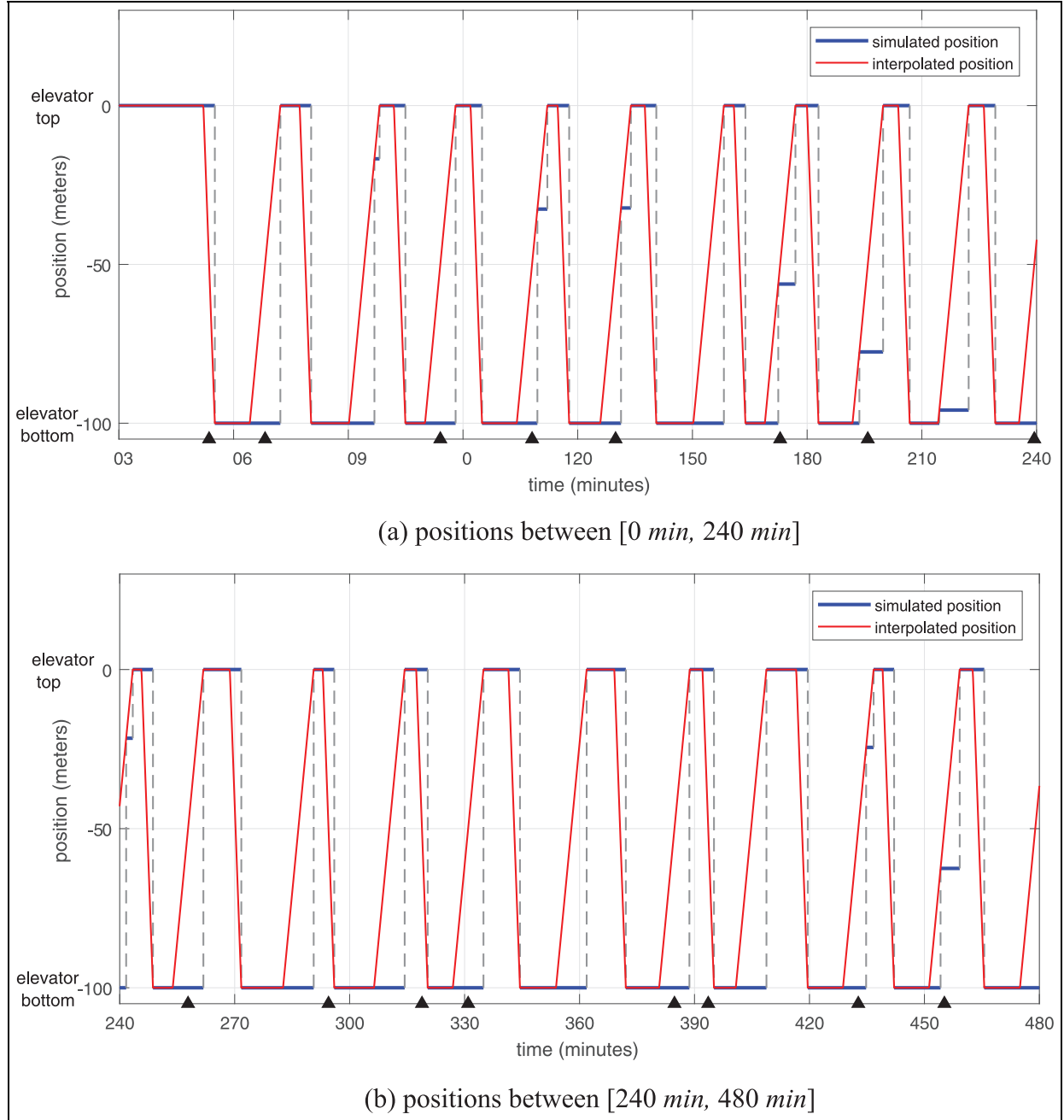
Figure 8. The state trajectory of the elevator in terms of position (the piecewise constant segments between the elevator top and the elevator bottom are the result of the elevator processing external events; each black triangle represents a time instant when a noisy observation of the elevator position is available; color online only).
