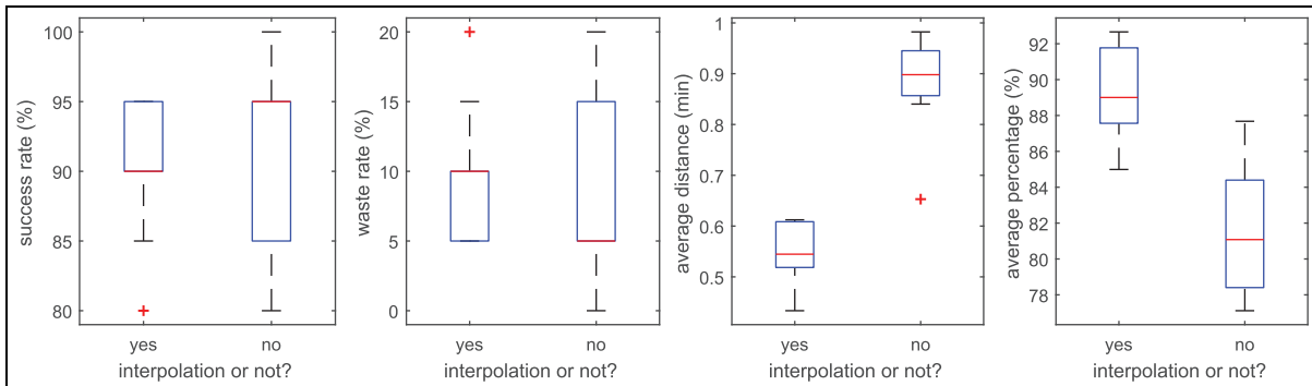
Figure 15. The influence of interpolation on the data assimilation results (noisy dataset ( \sigma_e = 3.0, \sigma_t = 3.0 ); N_p = 2000 ; 10 independent runs; color online only).
