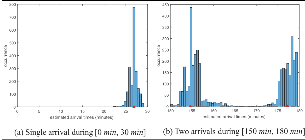
Figure 11. Histogram of estimated truck arrival times at the bottom of the vertical shaft during one step [(k-1)\Delta T, k\Delta T] , where \Delta T = 30 min (each red triangle represents a truck arrival in ground truth; color online only).
