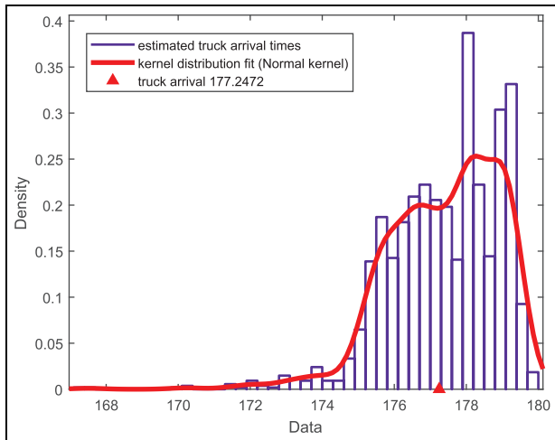
Figure 12. Fitting a kernel probability distribution using the Normal kernel to truck arrival times in one cluster (this group of data belongs to the cluster on the right-hand side in Figure 11(b); the red triangle represents a truck arrival in ground truth; color online only).
