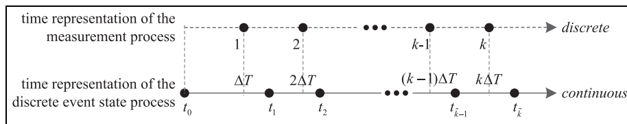
Figure 3. Time representation of the discrete event state process (each black dot indicates a state update) and the (discrete time) measurement process (each black dot represents the arrival of a measurement).
