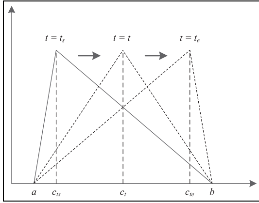
Figure 7. Triangular distribution with varying modes.
