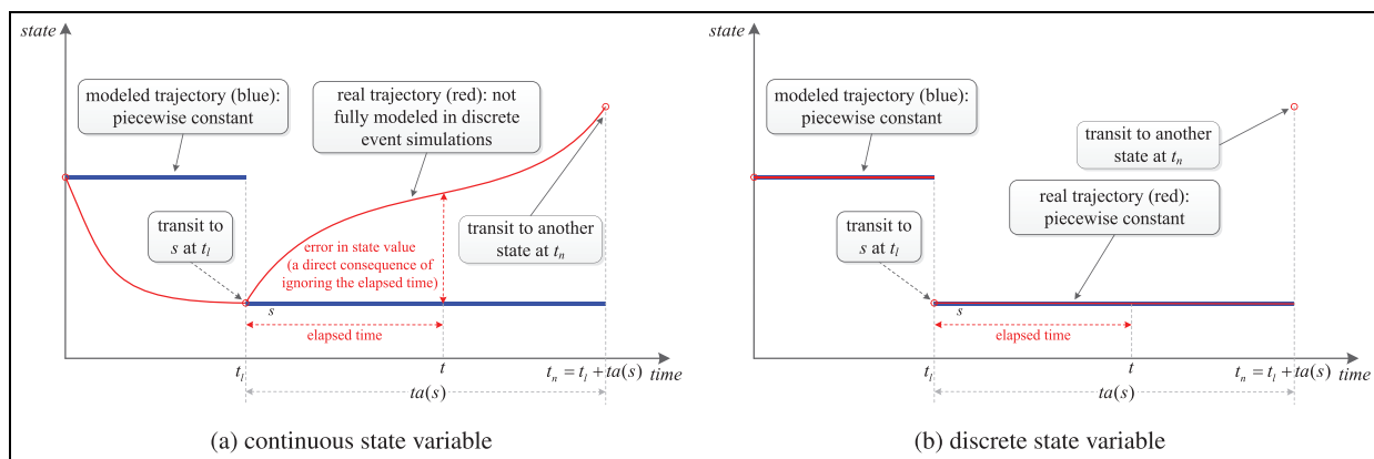
Figure 1. Discrete event simulation of continuous and discrete state variables. (Color online only.)
