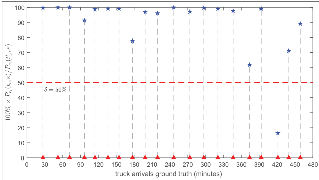
Figure 14. The match criterion 100\% \times P_{c_i}(t_i, \epsilon) / P_{c_i}(t_{c_i}^*, \epsilon) (each red triangle represents a truck arrival in ground truth; color online only).
