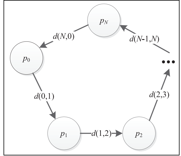
Figure 9. The phase transition graph.
