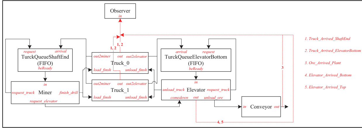
Figure 6. The Discrete Event System Specification model of the gold mine system. FIFO: first-in, first-out. (Color online only)
