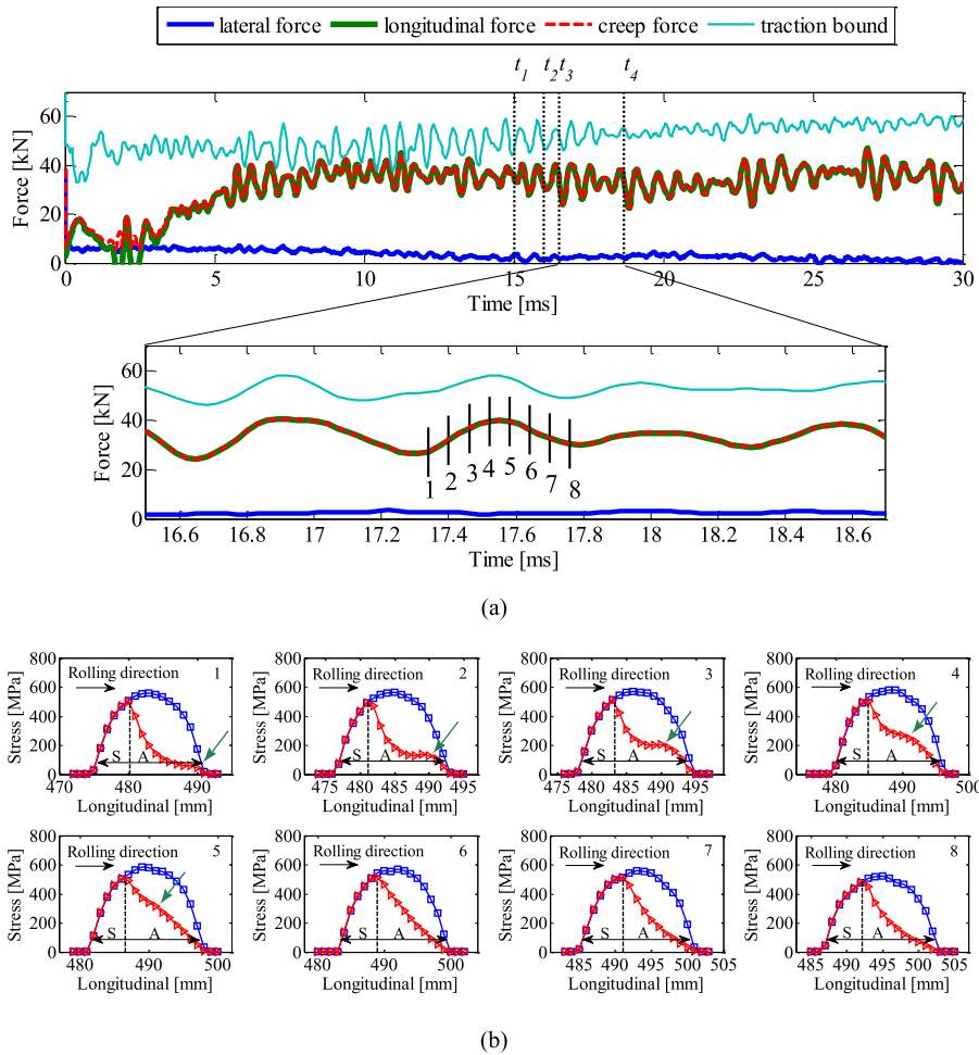
Fig. 5. Periodic surface stress distributions for simulation case 1. (a) Magnified view (within the solution zone) of the time histories of the contact forces for simulation case 1; (b) stress distributions calculated at corresponding time points denoted by 1–8 in (a) (blue curve: traction bound; red curve: surface shear stress; A: adhesion region; and S: slip region; the green arrows indicate the position of the moving local peak). (For interpretation of the references to color in this figure legend, the reader is referred to the web version of this article.)
