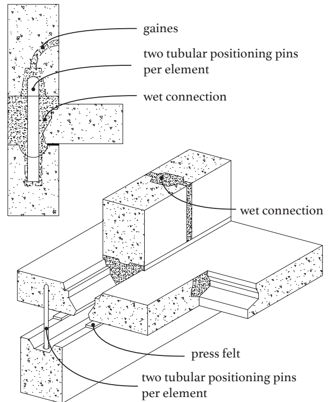
Figure 1.2.8: Construction details
