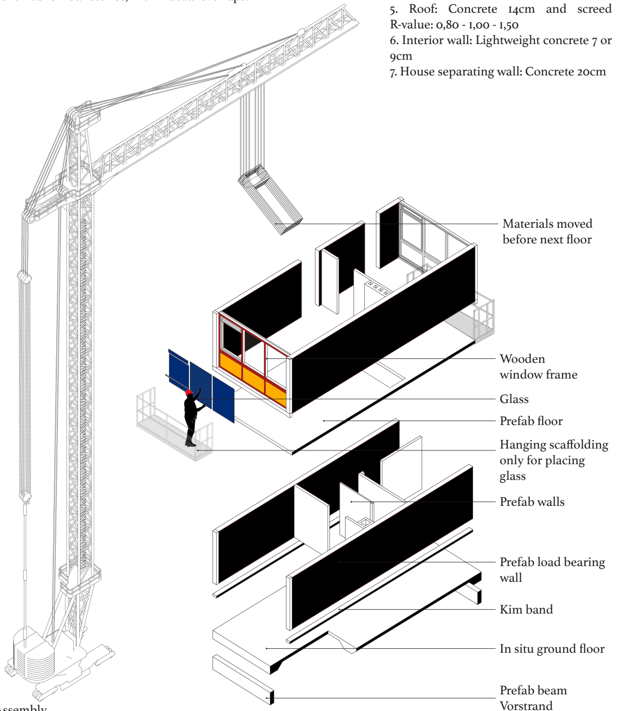
Figure 1.2.9: Assembly
