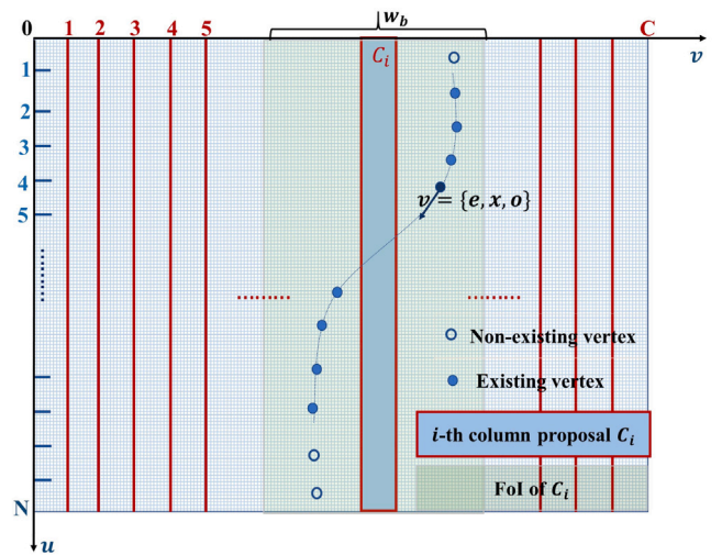
Fig. 2. Schematic diagram of the column proposal-based formulation for lane markings. C initial column proposals are displayed in the horizontal direction. Each polyline in the FoI of a proposal has a buffer width of w_b and a maximum of N sampled points in the vertical direction. The existence e , coordinate x , and orientation o of each vertex v are to be estimated.
