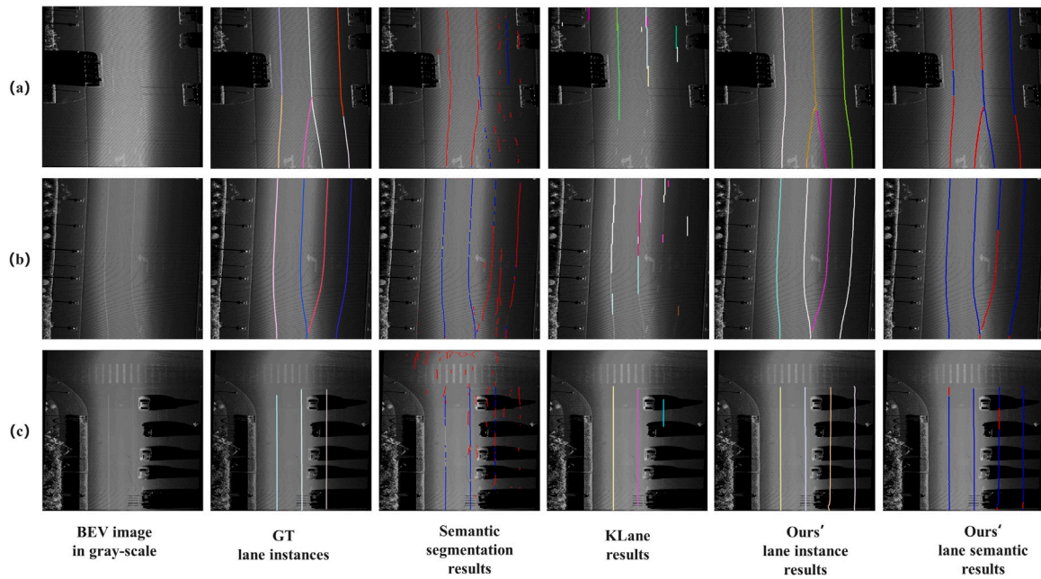
Fig. 12. Qualitative comparison results between the proposed method and classic FPN-based semantic segmentation (Lin et al., 2017) and KLane (Paek et al., 2022). For clarity, the lane markings are overlaid on grayscale images converted from the original BEV images. Lane instances are randomly colored. In terms of lane semantics, dashed lane markings are depicted in red, while continuous lane markings are in blue. (For interpretation of the references to color in this figure legend, the reader is referred to the web version of this article.)
