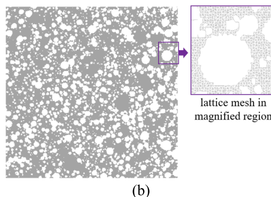
Fig. 6. (a) overlay procedure for a 2D lattice mesh; (b) 2D lattice mesh of foamed concrete after the overlay procedure using X-CT image [44].
