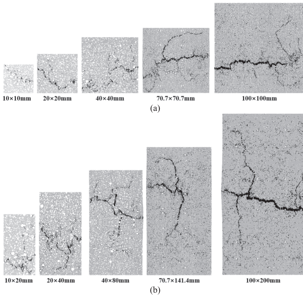
Fig. 12. Typical crack pattern of WD700 specimens at the failure stage: (a) Slenderness ratio = 1; (b) Slenderness ratio = 2.
