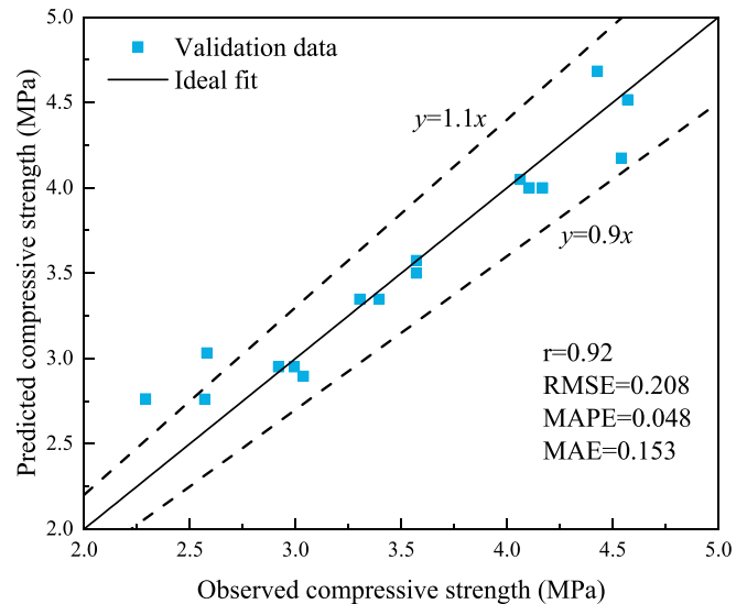
Fig. 17. Comparison of observed and predicted results.
