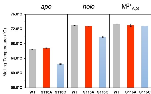
Figure 5. Protein melting temperatures. Thermal unfolding was investigated by nano-differential scanning fluorimetry for variants of SwHKA under different conditions. The holoenzyme state could correspond to both M^{2+}_R and M^{2+}_{A,S} . Conditions: SwHKA (5 mg mL -1 ), MgCl_2 (10 mM), hydroxyypyruvate (20 mM), in Hepes buffer (20 mM, pH 7.5).
