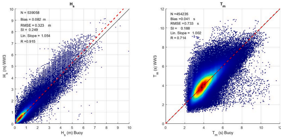
Fig. A.2. Scatter plots of the measured and modelled significant wave height ( H_s ) and the mean period ( T_m ) from in-situ wave buoys employed in the current study, using the source term parameterization T405 with the optimum value of \beta_{max} = 2.25 . The different error metrics (Bias, RMSE, SI, Pearson correlation R and the linear slope) are shown in both panels. The red dashed line, shown in each panel, represents the slope of the linear regression. The colour intensity corresponds to the density of data.
