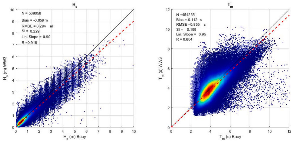
Fig. A.3. The same as Fig. A.2 but using the default value of \beta_{max} = 1.55 .
