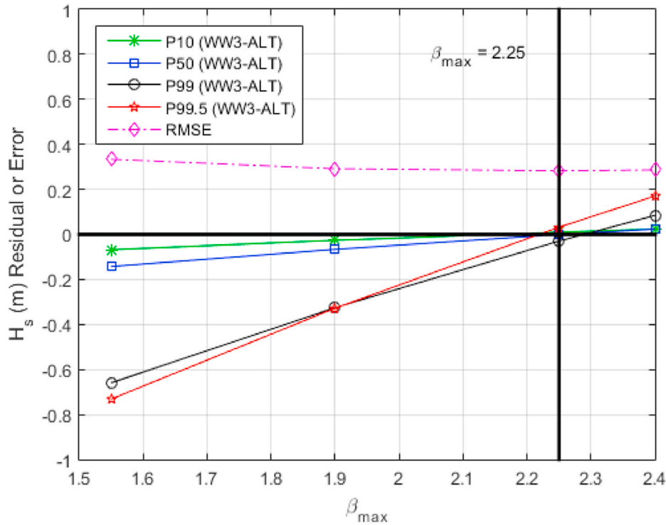
Fig. 3. Optimization of the \beta_{max} parameter in WW3 using model results and altimeter observations of H_s for the year 2011. The green, blue, black and red lines are, respectively, the 10th, 50th, 99th and 99.5th percentiles of H_s residual, i.e., the H_s from WW3 minus the H_s from altimeter. The magenta dashed line represents the root mean square error. The optimum \beta_{max} value is specified by the vertical black line.
