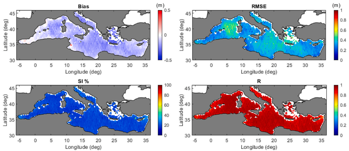
Fig. A.6. Spatial distributions of the Bias (Bias panel), the RMSE (RMSE panel), the scatter index (SI % panel), and the correlation coefficient (R panel) in H_s using the default value of \beta_{max} = 1.55 . The performance of the MS hindcast is evaluated using, as benchmark, the SSSCI altimeter data of H_s from 1991 to 2018.
