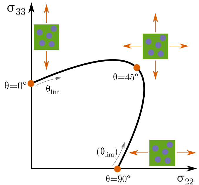
Fig. 12. Illustration of a biaxial yield envelope. The angle \theta defines the ratio between the two stress components. When training surrogates, \theta_{lim} is used to define the bounds of the training space.
