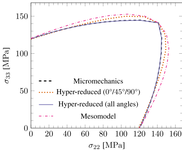
Fig. 17. Biaxial yield envelopes obtained with a hyper-reduced model trained on pure stress cases plus \theta = 45^\circ and with another one trained with all values of \theta . The mesomodel envelope is shown for comparison.
