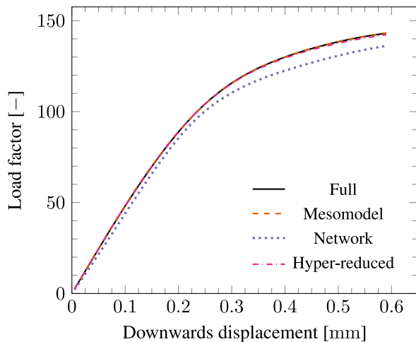
Fig. 28. Load-displacement curves for the short beam FE^2 example. Predictions made with all three surrogate modeling strategies are shown. The analysis is stopped before the perfect plasticity plateau due to non-convergence of the full-order FE^2 model.
