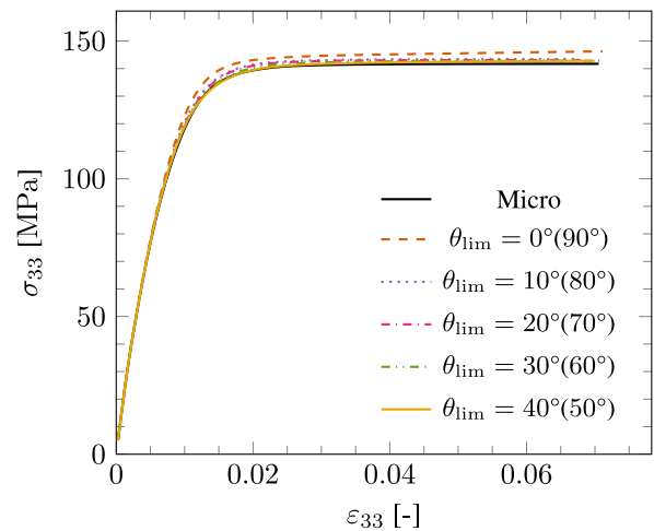
Fig. 13. Hyper-reduced model predictions of the biaxial transverse tension response when \theta = 45^\circ . Curves from models trained only on pure stress states ( \theta_{lim} = 0 ) as well as models retrained with additional biaxial cases ( \theta_{lim} > 0 ) are shown.
