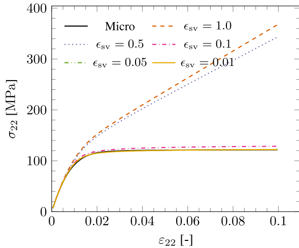
Fig. 3. Hyper-reduced model trained with pure stress states. Predictions improve as the truncation tolerance \epsilon_{sv} is reduced.
