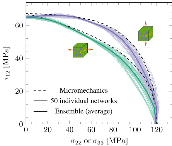
Fig. 21. Biaxial yield envelopes for the \sigma_{22(\text{33})} - \tau_{12} combination obtained by 50 bootstrapped networks trained with pure stress cases plus the biaxial case \theta = 45^\circ .
