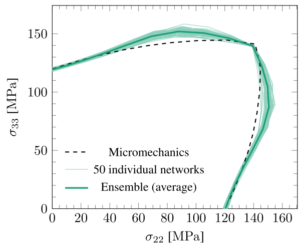
Fig. 15. Biaxial yield envelopes obtained by 50 different bootstrapped networks trained with pure stress states plus the biaxial case \theta = 45^\circ .
