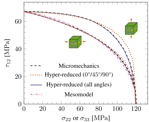
Fig. 23. Biaxial yield envelopes ( \sigma_{22(\text{33})} - \tau_{12} ) obtained with a hyper-reduced model trained on pure stress cases plus \theta = 45^\circ and with one trained with all values of \theta . The mesomodel envelope is shown for comparison.
