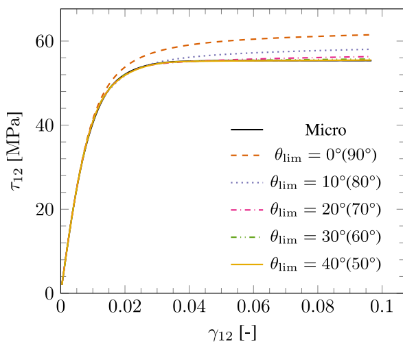
Fig. 18. Hyper-reduced model predictions of the biaxial \sigma_{22} - \tau_{12} response when \theta = 45^\circ . Curves from models trained only on pure stress cases ( \theta_{lim} = 0 ) as well as models retrained with additional biaxial cases ( \theta_{lim} > 0 ) are shown.
