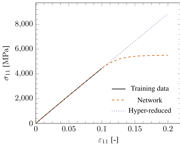
Fig. 10. Surrogate models used to predict material behavior outside of the strain range seen during training. The hyper-reduced model predicts the correct response, while the network shows an unphysical perfectly-plastic behavior.
