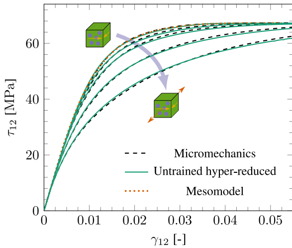
Fig. 24. Hyper-reduced model predictions for the biaxial \sigma_{11} - \tau_{12} response under various stress ratios. The model trained with only pure stress cases predicts these unseen scenarios remarkably well.
