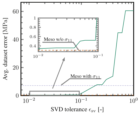
Fig. 4. Average absolute errors of the hyper-reduced model for the pure stress dataset.
