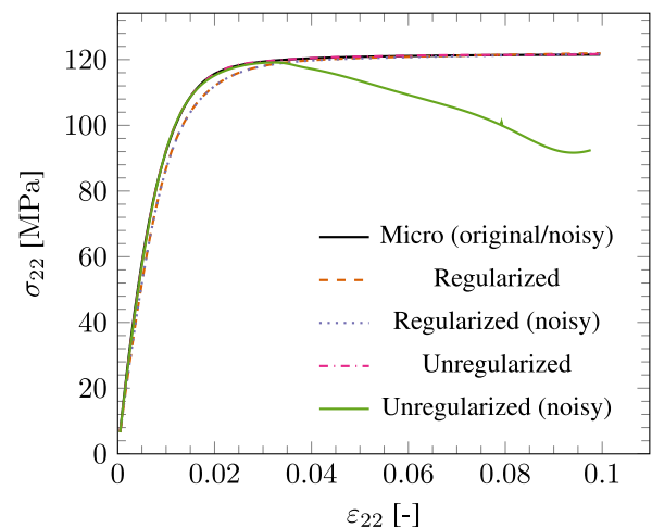
Fig. 9. Erroneous predictions by an unregularized neural network when making predictions on noisy strain values. The robustness introduced by the dropout layer alleviates the issue.
