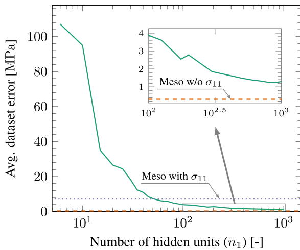
Fig. 8. Average absolute errors over the entire pure stress dataset for network models with different hidden layer sizes ( n_1 ).
