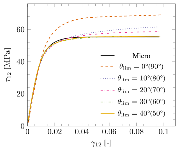
Fig. 19. Network model predictions of the biaxial \sigma_{22} - \tau_{12} response when \theta = 45^\circ . Curves from models trained only on pure stress cases ( \theta_{lim} = 0 ) as well as models retrained with additional biaxial cases ( \theta_{lim} > 0 ) are shown.
