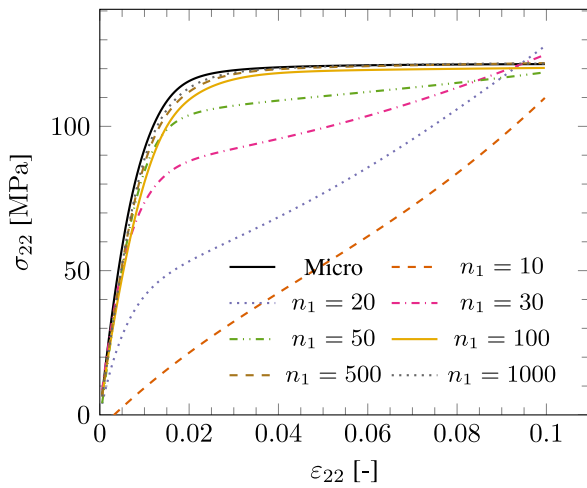
Fig. 7. Predictions of transverse stress made by neural network models with different hidden layer sizes ( n_1 ).
