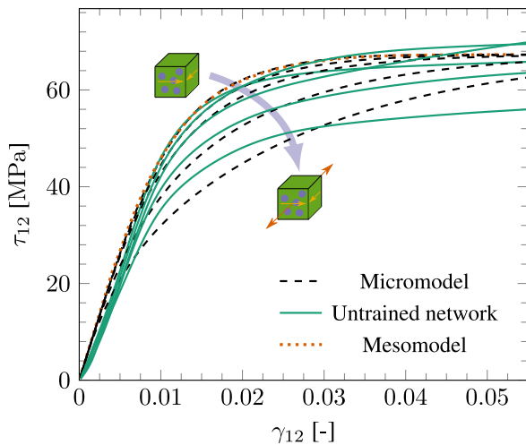
Fig. 25. Network model predictions for the biaxial \sigma_{11} - \tau_{12} response under various stress ratios. The curves are not reproduced well without additional network retraining.
