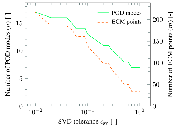
Fig. 5. Number of modes and integration points of the hyper-reduced model for different tolerances \epsilon_{sv} ( N = 21828 , M = 14176 ).
