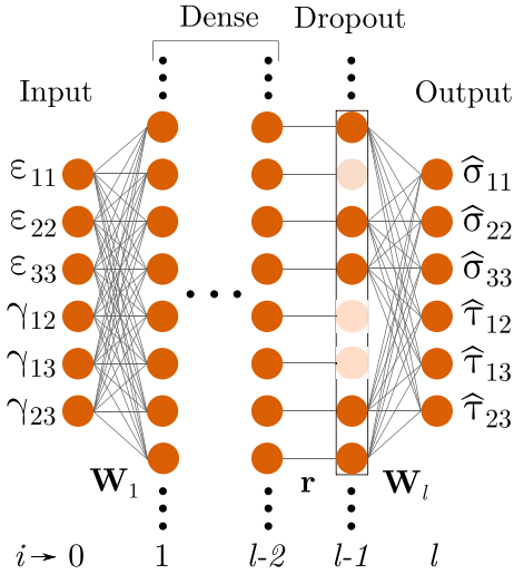
Fig. 2. A neural network acting as a surrogate constitutive model. An arbitrary number of dense neural layers is combined with a single dropout layer that regularizes model response.
