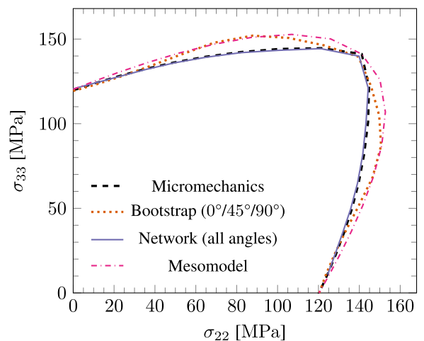
Fig. 16. Biaxial yield envelopes obtained with the bootstrapped network ensemble trained on pure stress cases plus \theta = 45^\circ and with a single network trained with all values of \theta . The mesomodel envelope is shown for comparison.
