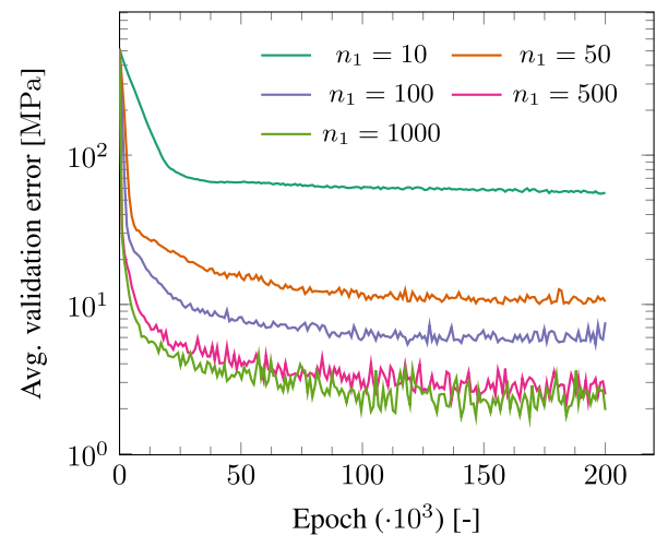
Fig. 6. Evolution of the average validation error during training of networks with different hidden layer widths ( n_1 ).
