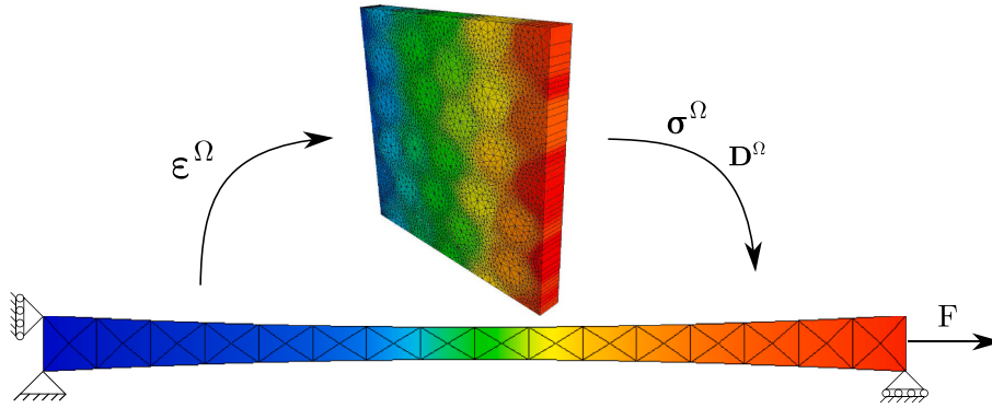
Fig. 1. The FE^2 approach: A concurrent link is established between meso and microscales.
