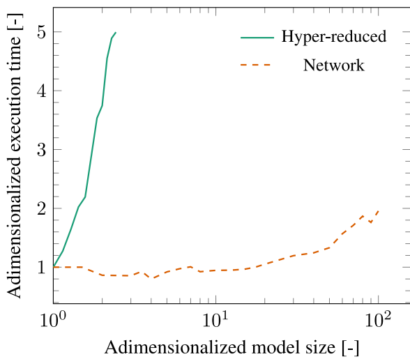
Fig. 11. Increases in execution time when model size ( n for hyper-reduced models and n_1 for network models) is increased.
