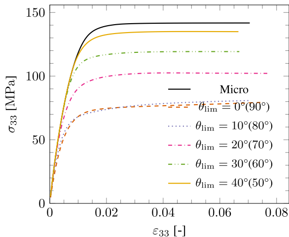
Fig. 14. Network model predictions of the biaxial transverse tension response when \theta = 45^\circ . Curves from models trained only on pure stress states ( \theta_{\text{lim}} = 0 ) as well as models retrained with additional biaxial cases ( \theta_{\text{lim}} > 0 ) are shown.
