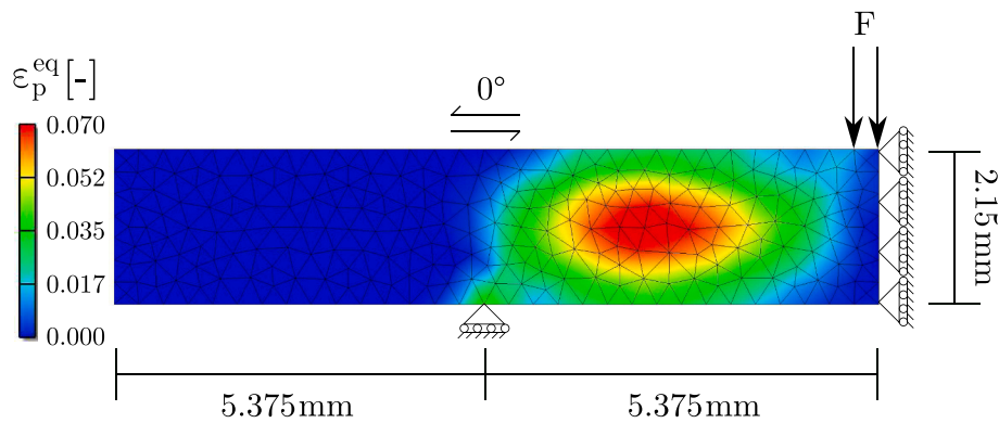
Fig. 27. Short-beam FE^2 example. Loads and boundary conditions are shown as well as the plastic strain field at the final time step.
