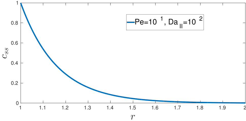
Fig. 3. Steady state concentration profile c_{ss} as function of r (Regime B) for a fixed value of Pe = 10^1 and Da_{||} = 10^2 .
