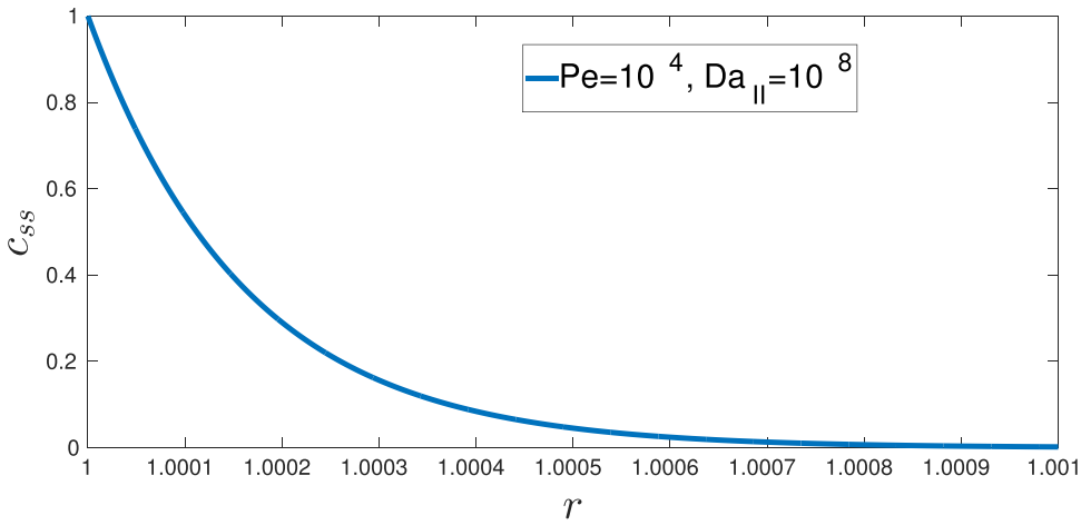
Fig. 4. Steady state concentration profile c_{ss} as function of r (Regime B) for a fixed value of Pe = 10^4 and Da_{||} = 10^8 . The figure seems similar to Fig. 3. Note, however, the different scale on the r -axis compared to Fig. 3.
