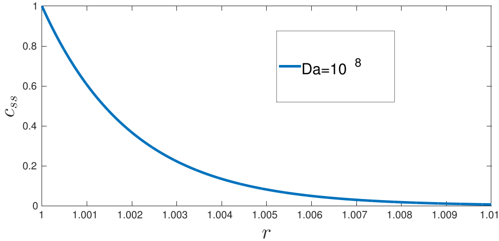
Fig. 2. Steady state concentration profile c_{ss} as function of r (Regime A) for a fixed value of Pe = 10^5 and Da_{II} = 10^8 . Note the different scale on the r -axis compared to Fig. 1.
