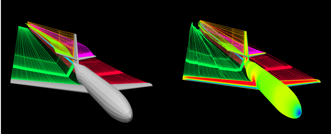
Fig. 3 Wake models before and after VSAERO analysis
