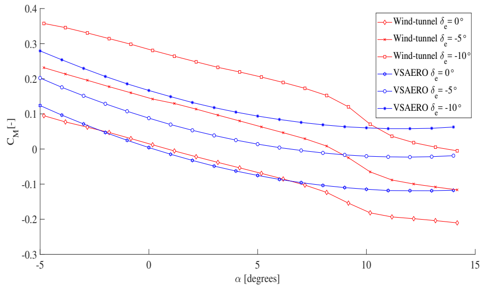
Fig. 7 Moment polar obtained from VSAERO and wind-tunnel test for different elevator deflections at 5 \times 10^5
