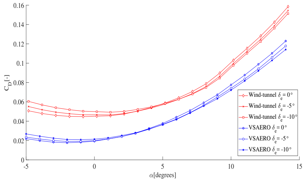
Fig. 6 Drag polar obtained from VSAERO and wind-tunnel test for different elevator deflections at Re = 5 \times 10^5
