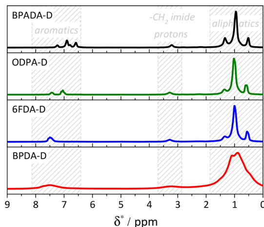
Figure 5. SS NMR one-pulse spectra, magic angle spinning (MAS) at 10 kHz, T_{exp} = T_{\tan \delta \text{ MAX}} + 120 °C.
