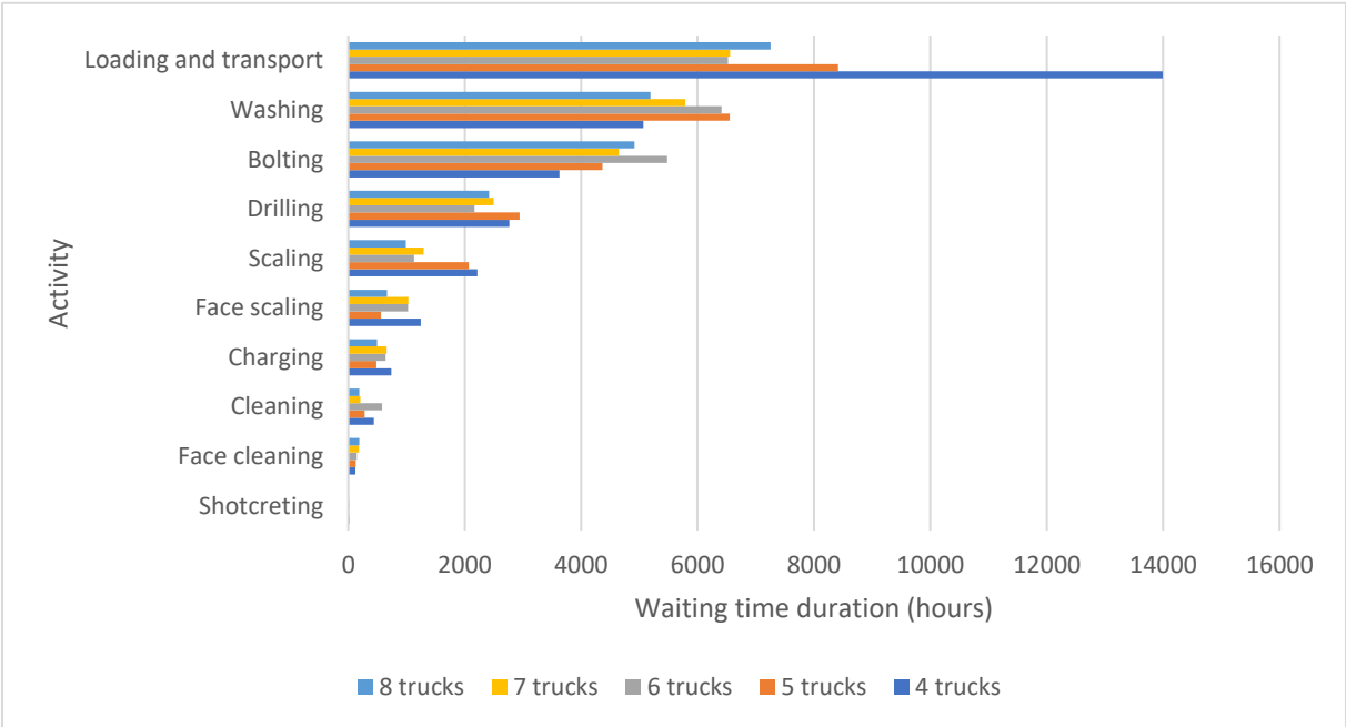
Figure 47: Waiting time duration change for different simulation scenarios.
