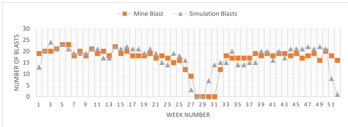
Figure 35: Number of blasts for the mine production and simulation on weekly basis.
