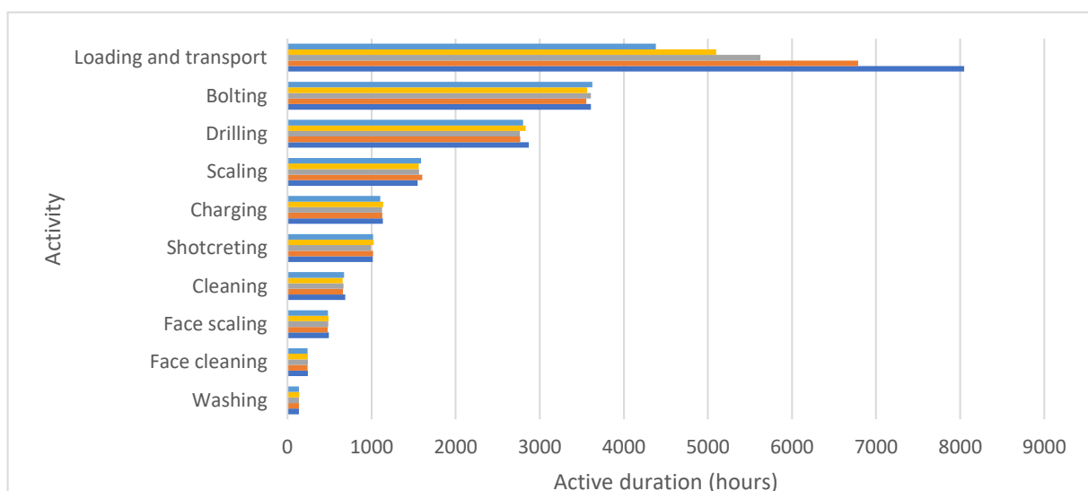
Figure 46: Active duration for each activity using different truck numbers over one year simulation period.
