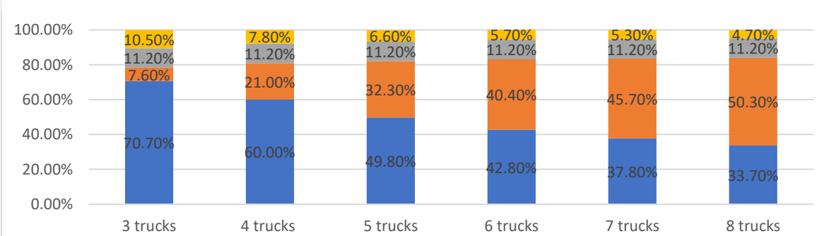
Figure 43 : Truck utilization for different numbers of trucks used in the simulation.
