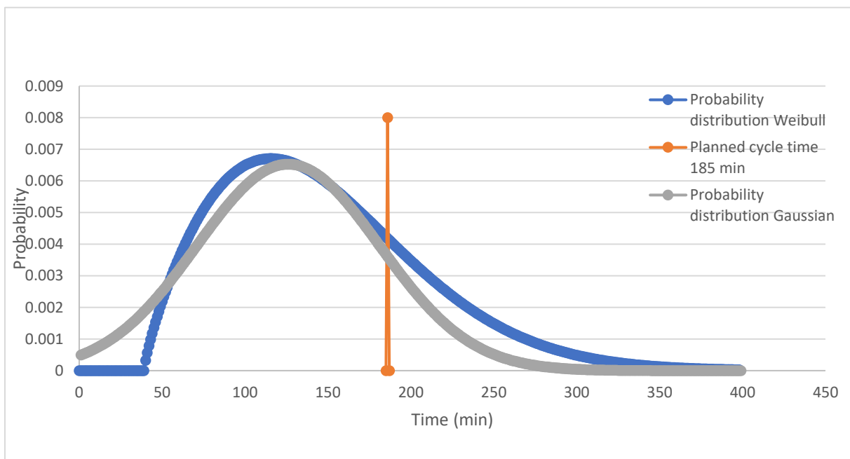
Figure 13: The data was fitted with a Weibull and Gaussian distribution. The collected data from the other mine is better in quantity and quality because it is continuously measured, but can unfortunately not be used for this simulation.
