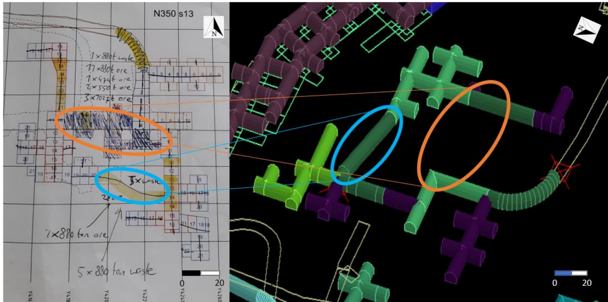
Figure 21: Corrective changes of the Simulation model. On the left side the mine plan with changes of the actual production, and on the right side the corrective changes in the Simulation model. The different colours represent different production sizes, and ore and waste material on which the simulation is based.
