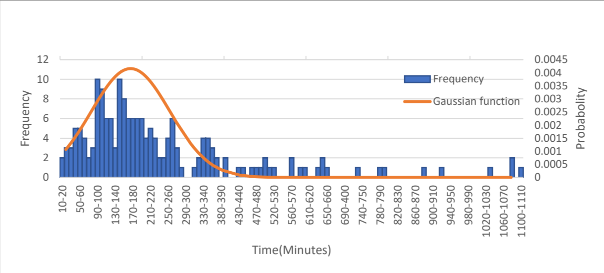
Figure 15 : Histogram showing the frequency distribution of the total drilling cycle time in minutes with a mean of 172.17 and standard deviation of 95.94 and fitted Gaussian distribution. From this picture it becomes clear that the distribution does not fit the data very well.
