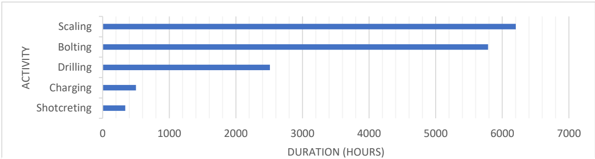
Figure 38: Total electrical engine hours measured over 2019 based on the Maximo software.
