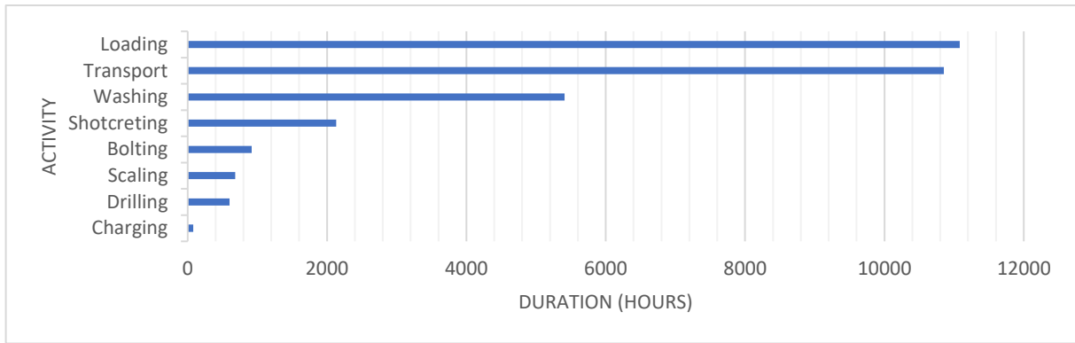
Figure 40 : Total diesel engine hours measured over 2019 based on the Maximo software.
