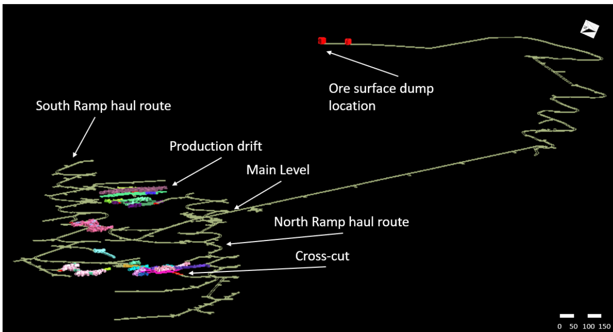
Figure 22: The mine layout of 2019 especially created for this simulation study in a CAT software program, and imported into SimMine simulation software. The North-ramp is connected to the surface ramp and North and South ramp are connected with one ramp on the main level. The South-ramp has no direct access to the surface.
