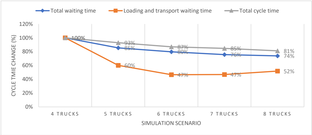
Figure 48: Cycle time change for the total cycle time, waiting time and loading and transport waiting time within the cycle.
