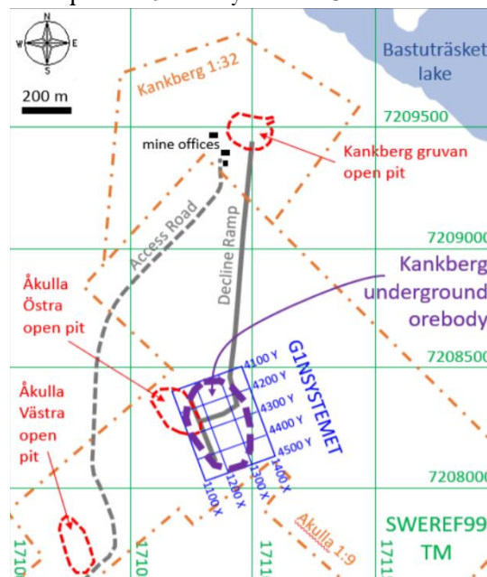
Figure 11: Simplified map of 2 km x 2.5 km area showing the Kankberg mining operation, with orebody outline, access and land rights (New Boliden).
