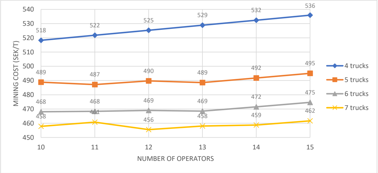
Figure 53 : Mining cost change for different number of operators and trucks.
