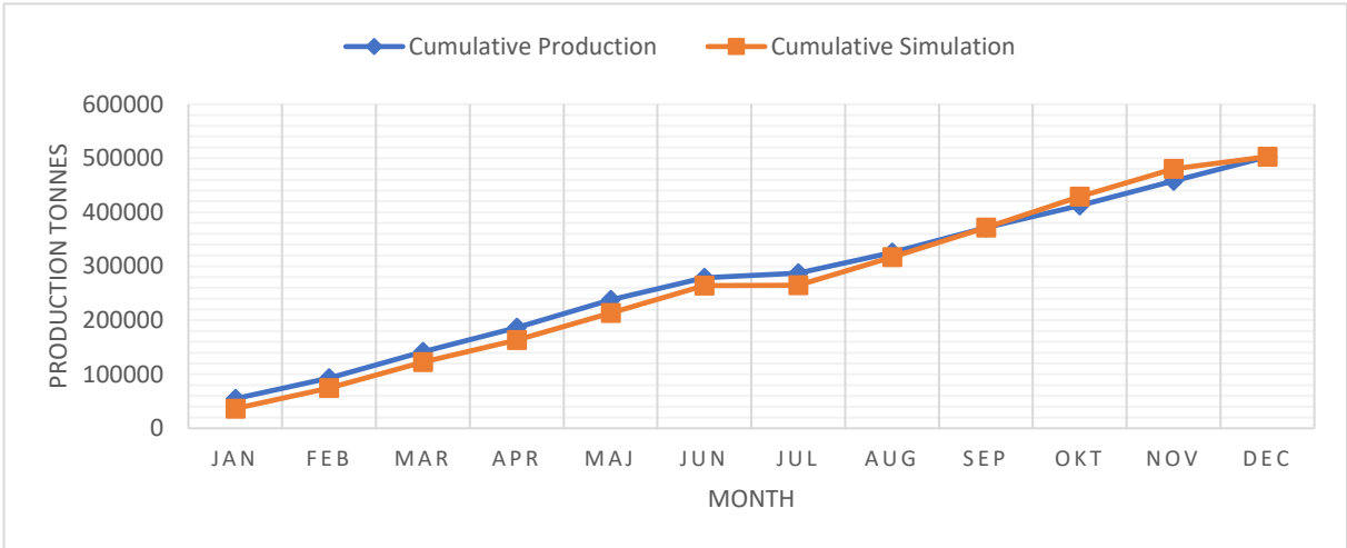
Figure 31: Cumulative production and cumulative simulation compared on monthly basis.
