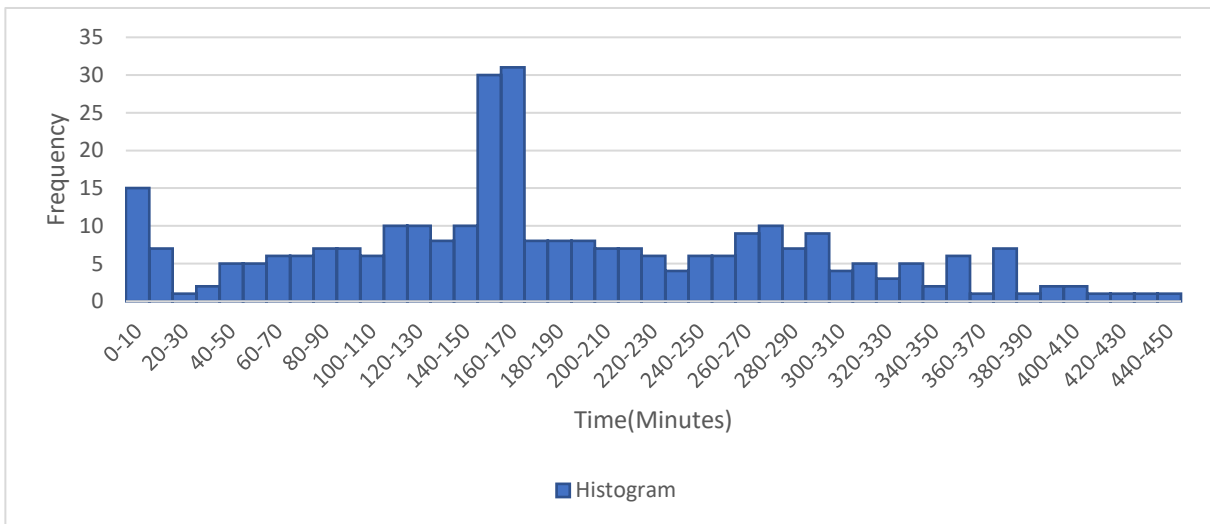
Figure 17: Histogram distribution of Certiq rock drilling activity duration, showing peak values around 160 and 170 minutes.
