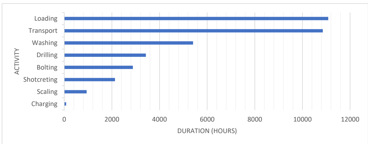
Figure 39 : Total engine hours, consisting out of the electrical hours and diesel hours.
