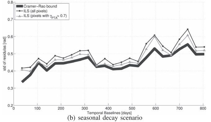
Fig. 12. Effect of the exclusion of unreliable estimates with \hat{\gamma}_{PTA} < 0.7 on the final precision of ILS SM-phase estimation for the two simulation scenarios. (a) Exponential decay. (b) Seasonal decay. By excluding the unreliable pixels, the standard deviations are reduced and approaching the CRB, confirming that the extended temporal coherence \hat{\gamma}_{PTA} can be used effectively for the final selection of DS with reliable phase estimation.
