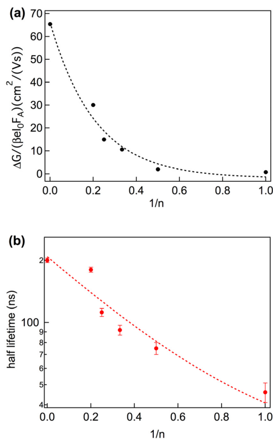
Figure 3. Photoconductivity (a) and half-lifetime (b) dependence of 2D perovskites on the thickness of the [(\text{MA})_{n-1}\text{Pb}_n\text{I}_{3n+1}]^{2-} slabs at room temperature. Excited at the emission wavelength. The dotted lines are a guide to the eye. In panel (a) the error bars are smaller than the symbols.
