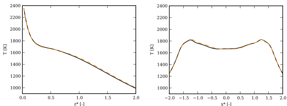
FIG. 5. Comparison of temperatures on x^* = 0 and z^* = 0.5 averaged over the period from 1.5 to 3.5 s, computed by dynamic LES (dashed, 2.5M cell mesh) and DNS (solid, 21M cell mesh).
