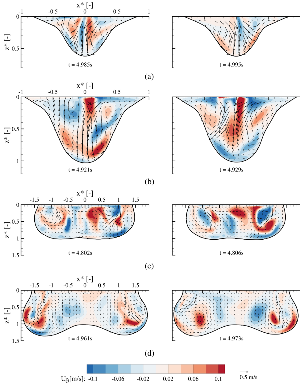
FIG. 12. Instationary in-plane ( x, z ) velocities in the y^* = 0 plane at two time instances indicated by vectors, and azimuthal velocities indicated by color contours: (a) Case 2, (b) case 3, (c) case 4, and (d) case 5. The figures in the left and right column have identical coordinates. (Multimedia view) [URL: http://dx.doi.org/10.1063/1.4953797.9 ] [URL: http://dx.doi.org/10.1063/1.4953797.10 ] [URL: http://dx.doi.org/10.1063/1.4953797.11 ] [URL: http://dx.doi.org/10.1063/1.4953797.12 ]
