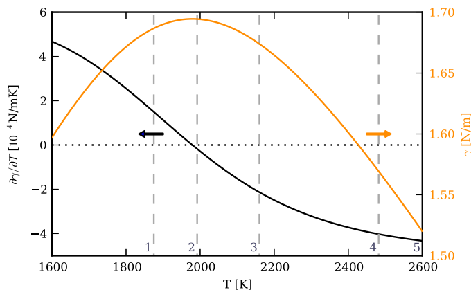
FIG. 2. Surface tension temperature coefficient. The critical temperature at which the sign change occurs is T_c = 1979 K. The vertical dashed lines indicate the maximum surface temperature reached in cases 1-5, as discussed later.
