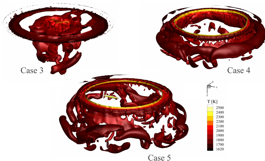
FIG. 17. Isosurface of Q at a time instance, colored according to temperature, visualizing vortex tubes in the unsteady liquid pools for case 3, case 4 and case 5. (Multimedia view) [URL: http://dx.doi.org/10.1063/1.4953797.13 ] [URL: http://dx.doi.org/10.1063/1.4953797.14 ] [URL: http://dx.doi.org/10.1063/1.4953797.15 ]
