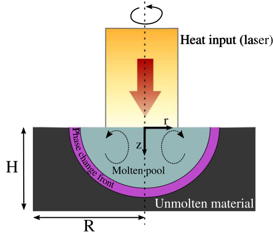
FIG. 1. Schematic representation of the studied problem.
