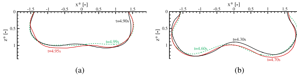
FIG. 13. Pool boundary oscillation observed in case 4 and 5. The oscillation frequency is significantly higher in case 4. (a) Case 4. (b) Case 5.
