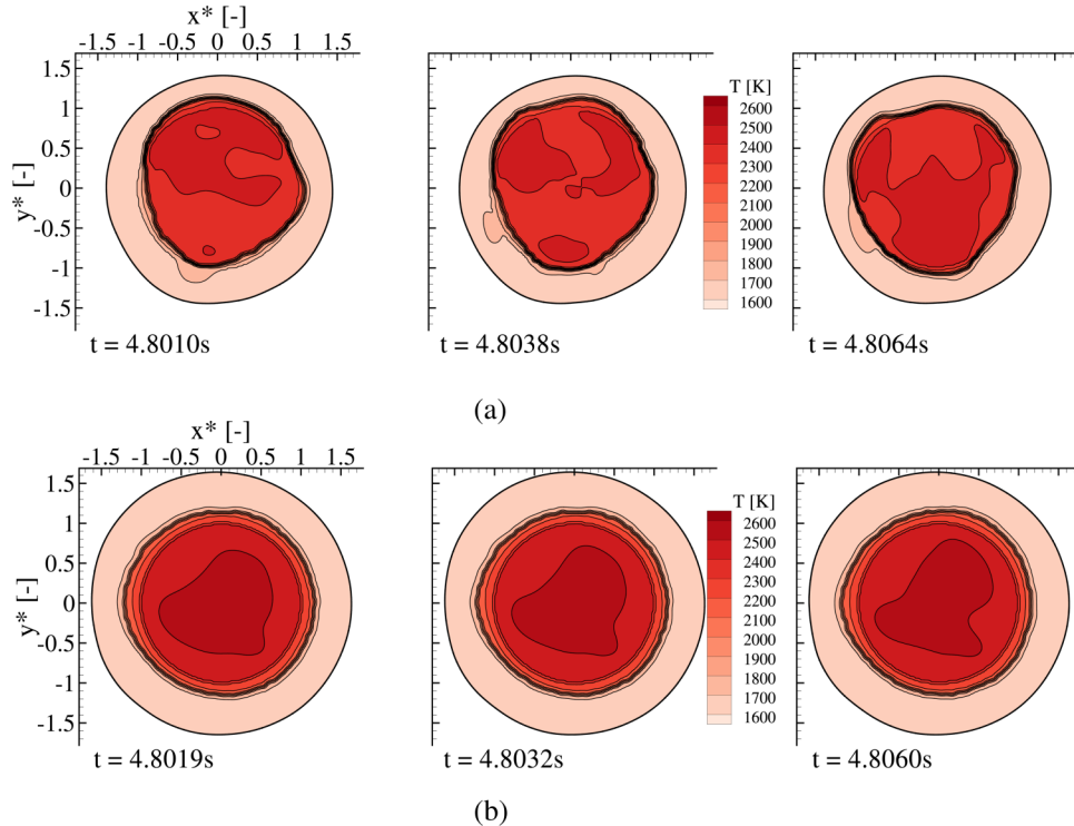
FIG. 9. Isotherms on the free surface for case 4 and 5, showing highly chaotic temporal behavior for case 4 and irregular, less intermittent behavior for case 5. (a) Case 4. (b) Case 5. All subfigures are plotted using the same coordinates. (Multimedia view) [URL: http://dx.doi.org/10.1063/1.4953797.7 ] [URL: http://dx.doi.org/10.1063/1.4953797.8 ]
