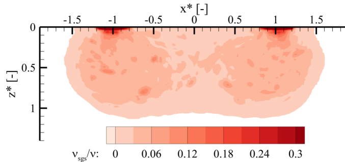
FIG. 4. Maximum values of the ratio of subgrid-scale and molecular diffusivity \nu_{sgs}/\nu in case 4, proving a well-resolved LES simulation.
