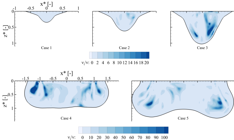
FIG. 16. Ratio of turbulent diffusivity over molecular diffusivity \nu_t/\nu in the y^* = 0 plane, based on turbulent kinetic energy and turbulence dissipation averaged over the 4.5 to 5 s period.
