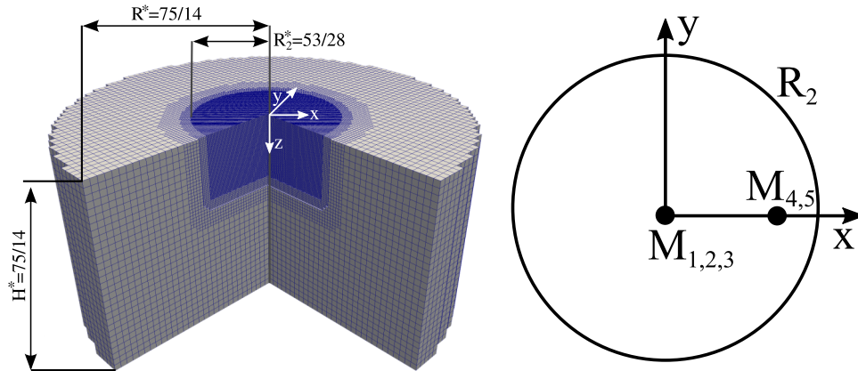
FIG. 3. 3D mesh, where one quarter of the domain has been clipped for visualization. The coarse outer mesh with a grid cell size of \Delta x^* = 0.178 is refined in three steps to the finest inner mesh with a grid cell size of \Delta x^* = 0.022 . The latter is too fine to be resolved in this figure. The sketch on the right shows monitoring point locations at a depth of z^* = 3/14 and radial distances of x^* = 0 ( M_{1,2,3} ) and x^* = 15/14 ( M_{4,5} ).
