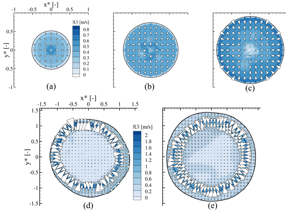
FIG. 6. Free surface flow with velocity vectors and contours of velocity magnitude, at t = 2 s for increasing laser power: (a) Case 1, (b) case 2, (c) case 3, (d) case 4, and (e) case 5. Subfigures (a)-(c) have identical coordinate systems, as do subfigures (d) and (e). (Multimedia view) [URL: http://dx.doi.org/10.1063/1.4953797.1 ] [URL: http://dx.doi.org/10.1063/1.4953797.2 ] [URL: http://dx.doi.org/10.1063/1.4953797.3 ] [URL: http://dx.doi.org/10.1063/1.4953797.4 ]
