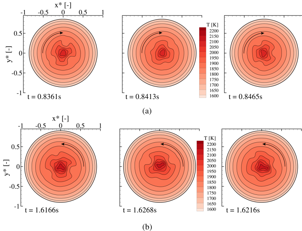
FIG. 8. Isotherms on free surface, case 3, showing clockwise rotation of the trefoil pattern at a certain time instance followed by counter-clockwise rotation at a later time. (a) Clockwise rotation. (b) Counter-clockwise rotation. All subfigures have identical coordinates. (Multimedia view) [URL: http://dx.doi.org/10.1063/1.4953797.6 ]
