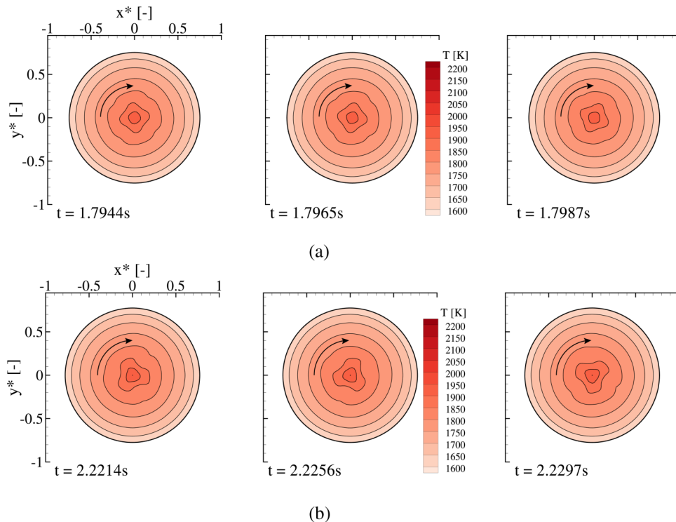
FIG. 7. Steady clockwise rotational motion of initially square and later trefoil shaped isotherm pattern on free surface, case 2. (a) Square pattern. (b) Trefoil pattern. All subfigures have identical coordinates. (Multimedia view) [URL: http://dx.doi.org/10.1063/1.4953797.5 ]
