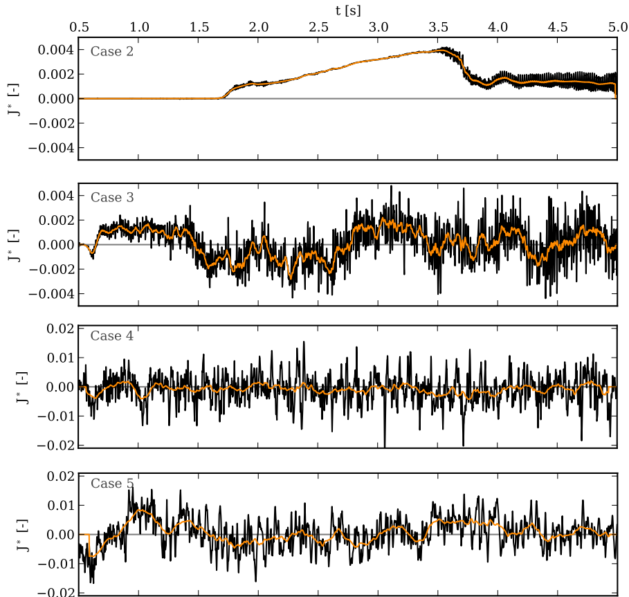
FIG. 10. Surface averaged angular momentum J^* of the free surface over time (orange line: moving average) for increasing laser power. Negative values translate to counter-clockwise motion.
