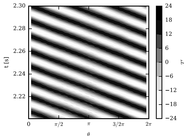
FIG. 11. Temperature fluctuation T' = T - \frac{1}{2\pi} \int_0^{2\pi} T d\theta at r^* = 0.143 in case 2, with \theta the azimuthal coordinate.
