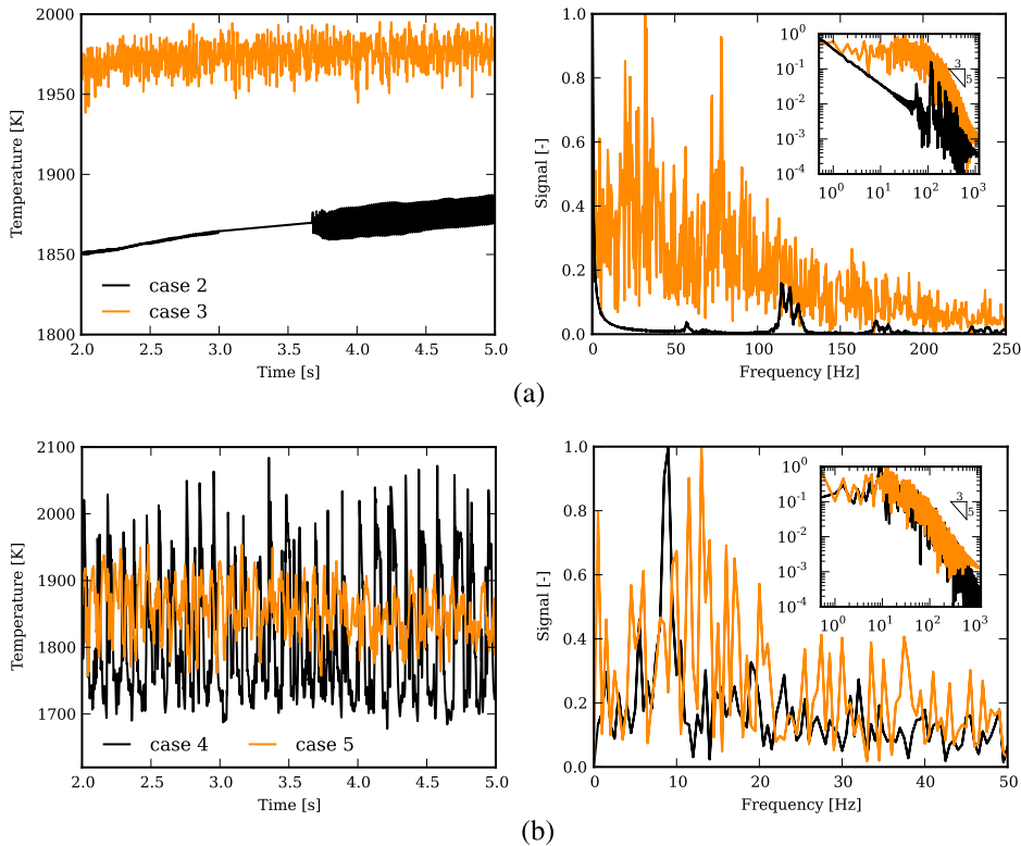
FIG. 15. Temperature signal and spectrum at monitoring points (see Fig. 3) for varying laser powers. The signal spectrum has been normalized with the respective maximum peak. (a) Case 2 and 3, point M_{1,2,3} . (b) Case 4 and 5, point M_{4,5} .
