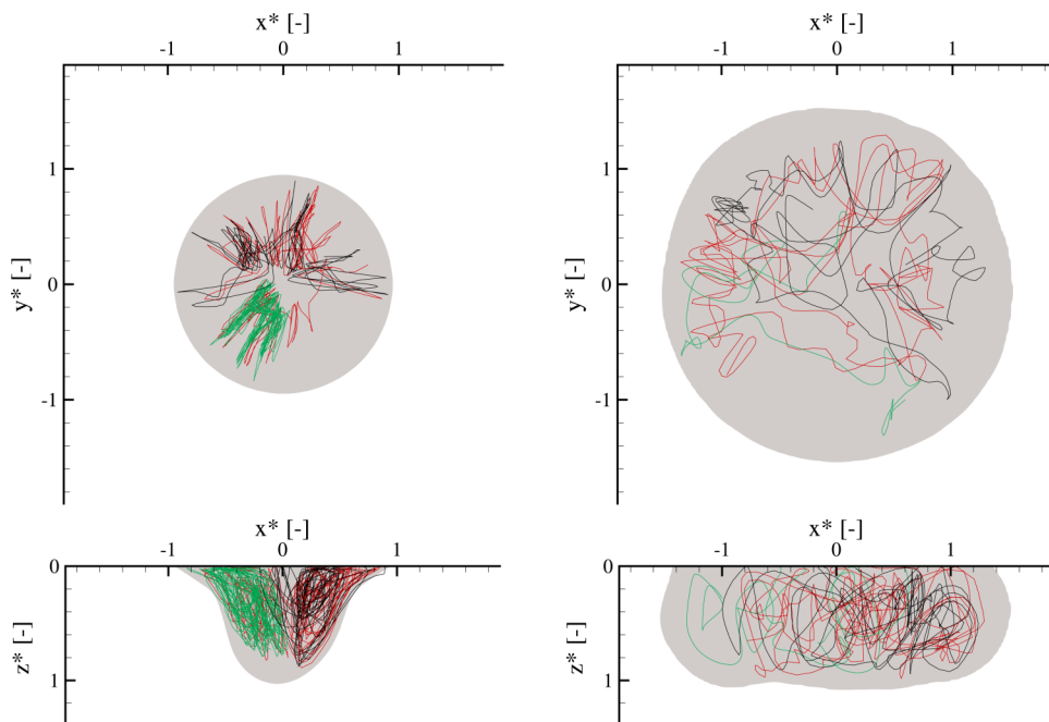
FIG. 14. Particle tracks for cases 3 (left half) and 4 (right half), showing regular unsteady motion for case 3 and chaotic motion for case 4.
