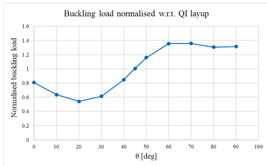
Fig. 17. Normalised buckling load with respect to the QI layup of [\pm\theta]_s layup.
