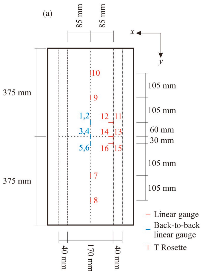
Fig. 10. (a) Strain gauge locations, orientation and identifier number on the stiffened panels; and (b) stiffened panels tested, showing strain gauges and Digital Image Correlation (DIC) speckling pattern.
