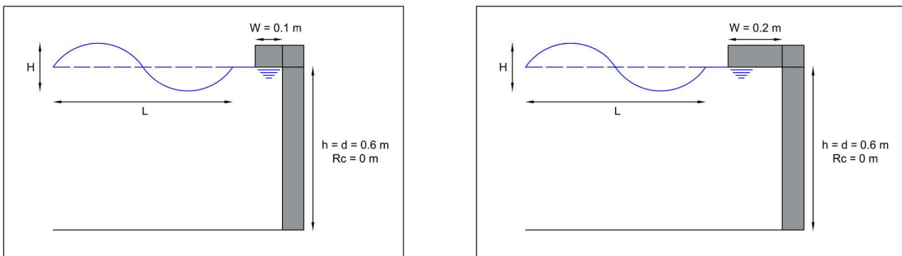
Fig. 7. Structure configurations. a) Shorter overhang.
