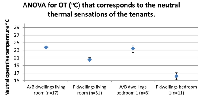
Fig. 7. ANOVA single factor for the operative temperatures that correspond to the neutral thermal sensations of the tenants.
