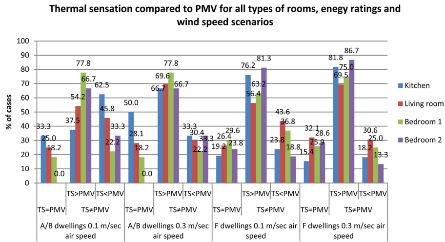
Fig. 10. Thermal sensation compared to PMV for all types of rooms, energy ratings and wind speed scenarios.
