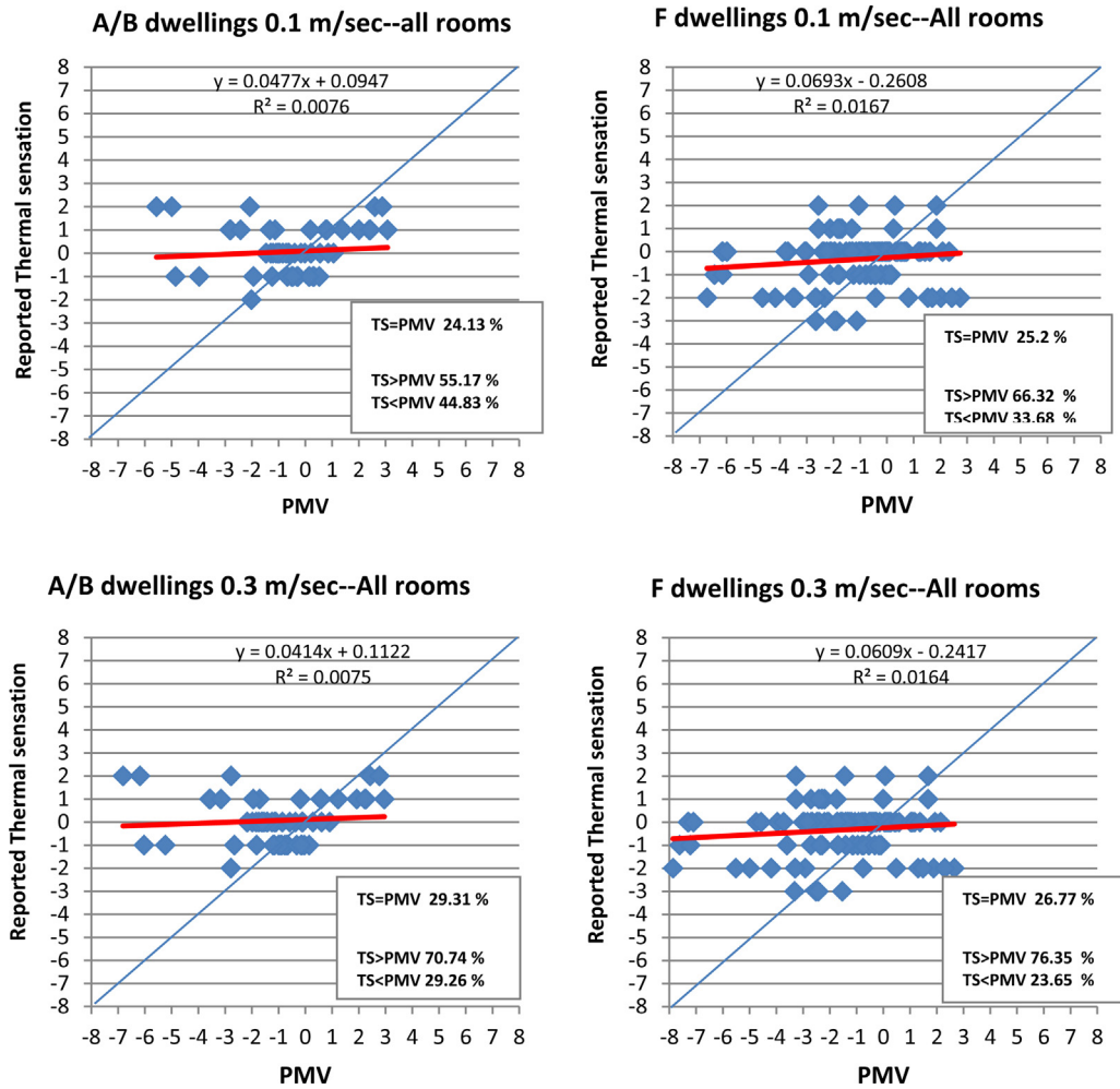
Fig. 9. Plots of reported thermal sensation against PMV for A/B and F dwellings, at air speeds of 0.1 m/sec and 0.3 m/sec (blue line TS = PMV, red line = regression line). (For interpretation of the references to colour in this figure legend, the reader is referred to the web version of this article.)
