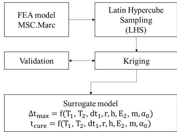
Fig. 2. Surrogate model construction methodology.
