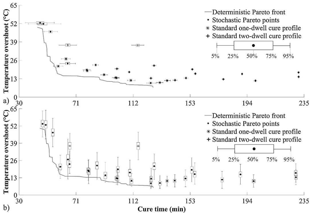
Fig. 10. Pareto front of stochastic and deterministic multi-objective optimisation (a) cure time box plots; (b) temperature overshoot box plots.
