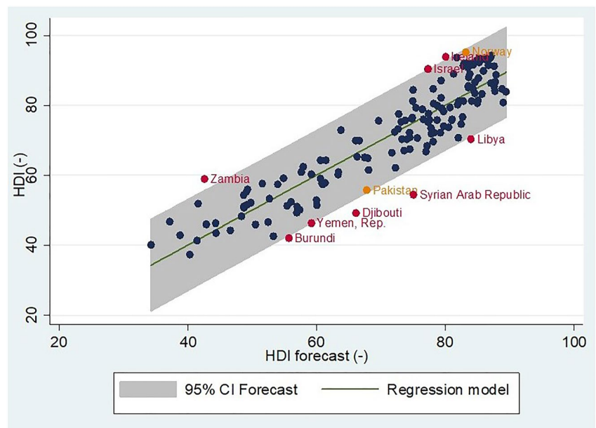
Figure 5. Observed against modeled HDI. Countries labeled in red are outside the 95% model prediction interval, countries labeled in orange are in the limit of the prediction interval. A mathematical description for the interval estimation is available in Supporting Information S1 (Text S2). A time-dynamic version of this model is available online.
