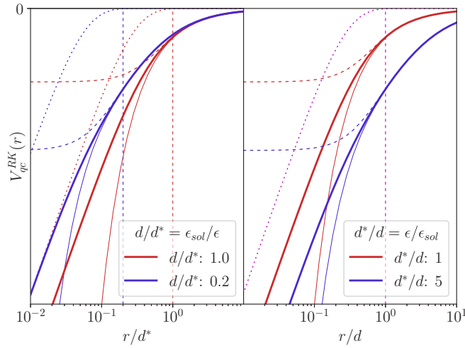
FIG. 6. Real-space dependence of the quantum-confined Rytova-Keldysh potential as a function of r/d^* (left) and r/d (right), computed by Fourier transforming Eq. (21). The two contributions V_<(r) and V_>^{RK}(r) are represented by dotted and dashed lines, respectively. The thin solid lines correspond to V^{RK}(r) , for each value of d/d^* = \epsilon_{\text{sol}}/\epsilon (left) and d^*/d = \epsilon/\epsilon_{\text{sol}} (right). The red line (bottom one on the left, top one on the right, d/d^* = 1 ) is computed using the quantum-confined Coulomb potential, and thus is the same as that shown in Fig. 5. Left: The vertical dashed lines correspond to the points r/d^* = d/d^* . Right: The vertical dashed magenta line corresponds to r/d = 1 .
