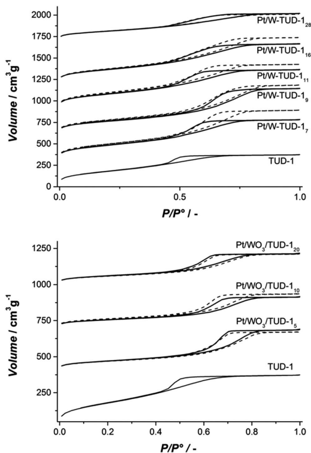
Fig. 1 (Top) isotherms of Pt/W-TUD-1 samples (bold) and W-TUD-1 samples (dashed); (bottom) isotherms of Pt/ \text{WO}_3/\text{TUD-1} samples (bold) and \text{WO}_3/\text{TUD-1} samples (dashed).
