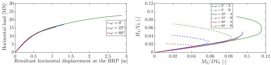
(a) horizontal force-displacement response at the hull (b) horizontal-moment spudcan load paths ( H_3/V_0 - M_2/DV_0 )
