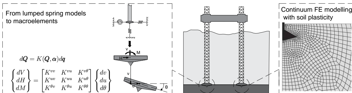
Figure 2: Lumped (left) vs continuum (right) modelling of soil-spudcan interaction.
