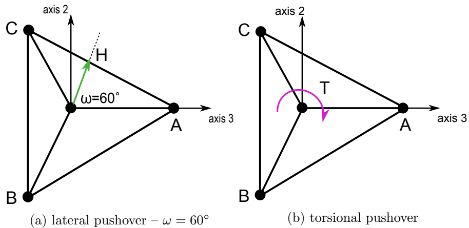
Figure 17: Loading conditions for additional pushover analyses.
