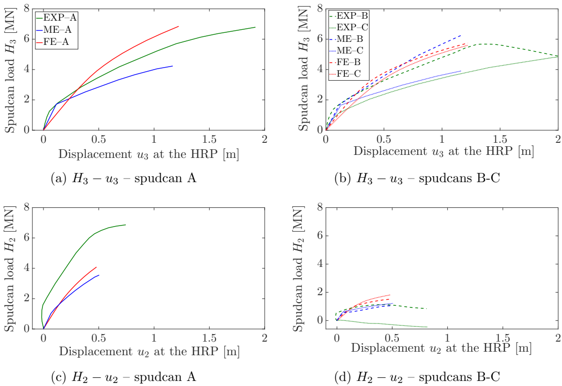
Figure 14: Spudcan force-displacement responses during misaligned pushover.
