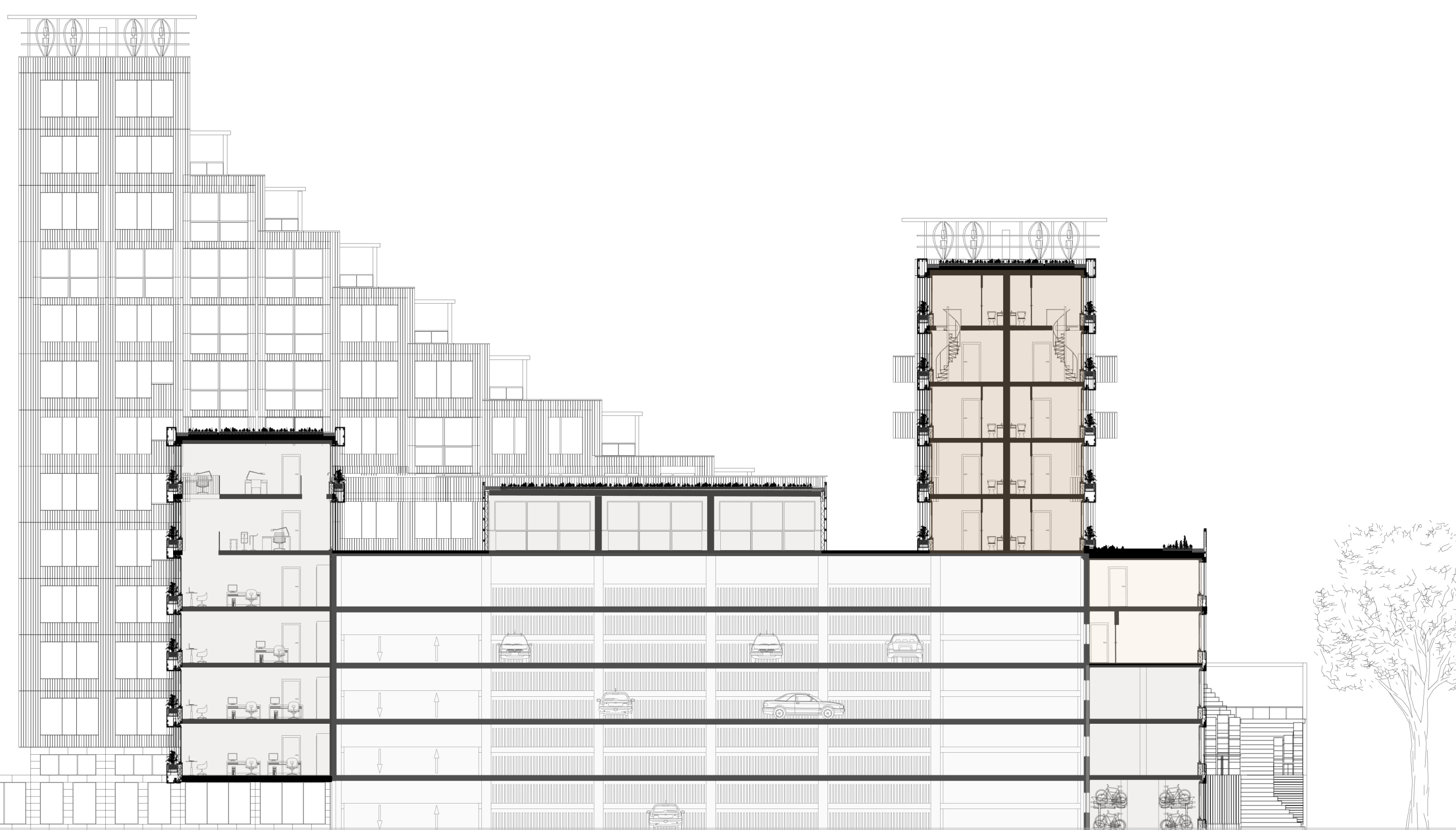
East-West section 1:200
