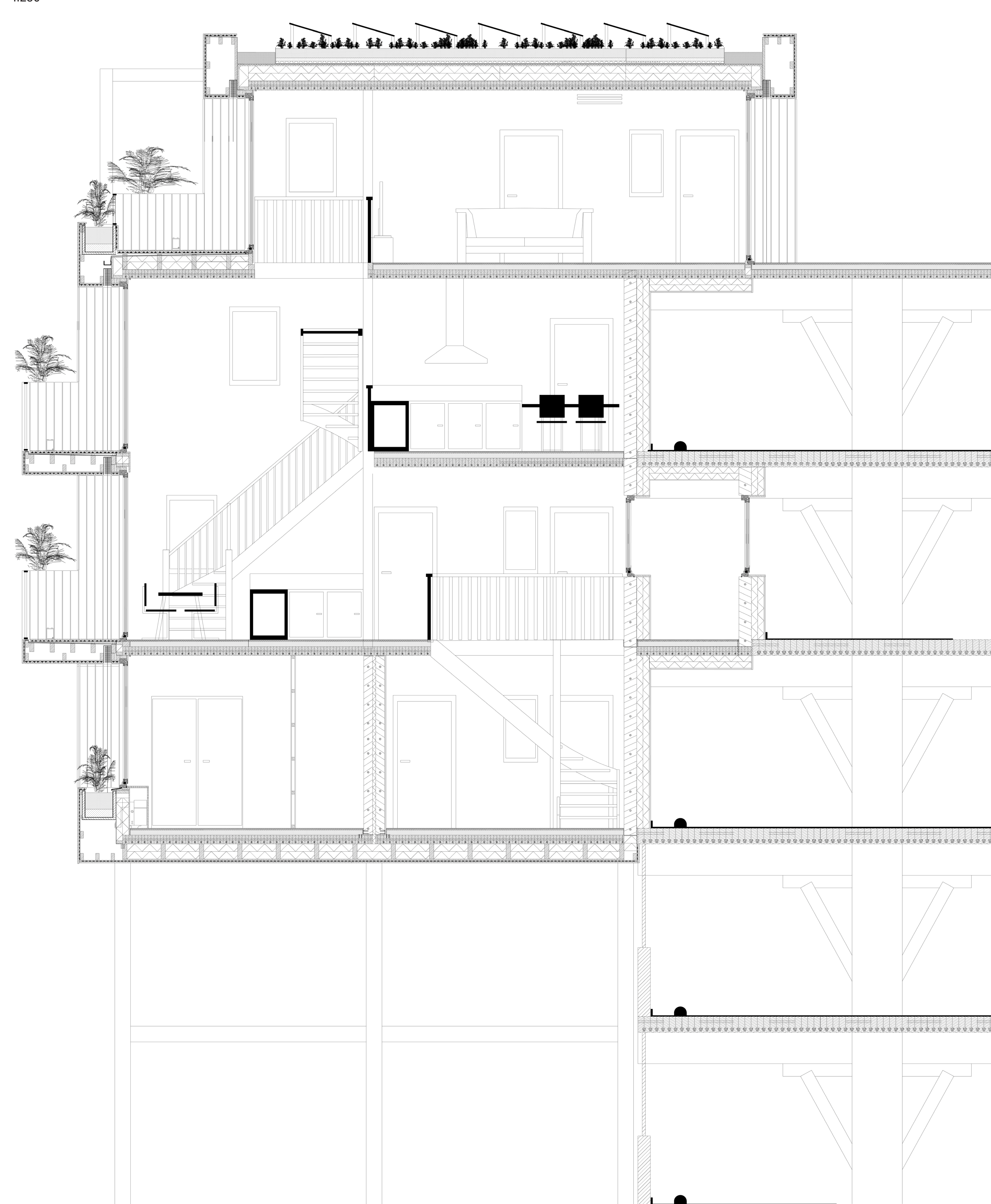
Regular cluster section 1:250
