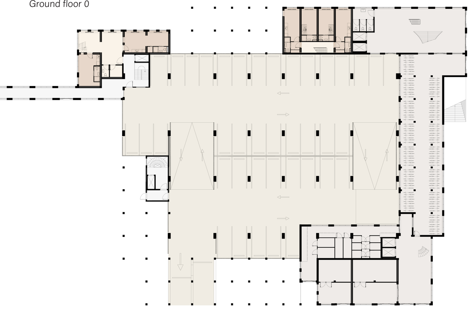
Floor plans 1:200 Ground floor 0
