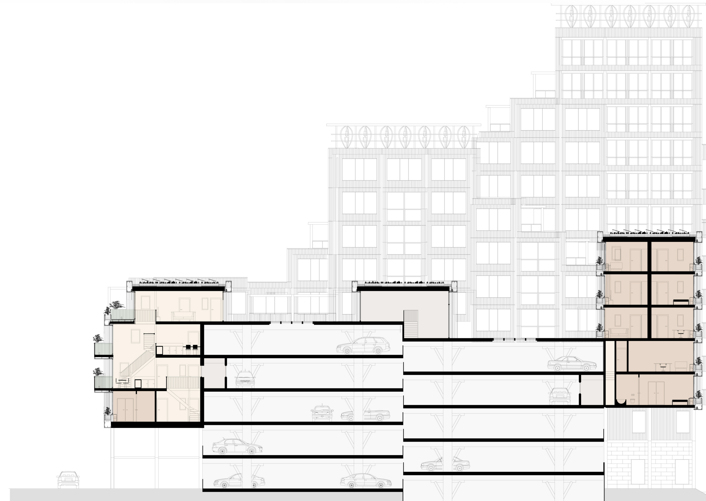
North-South section 1:200
