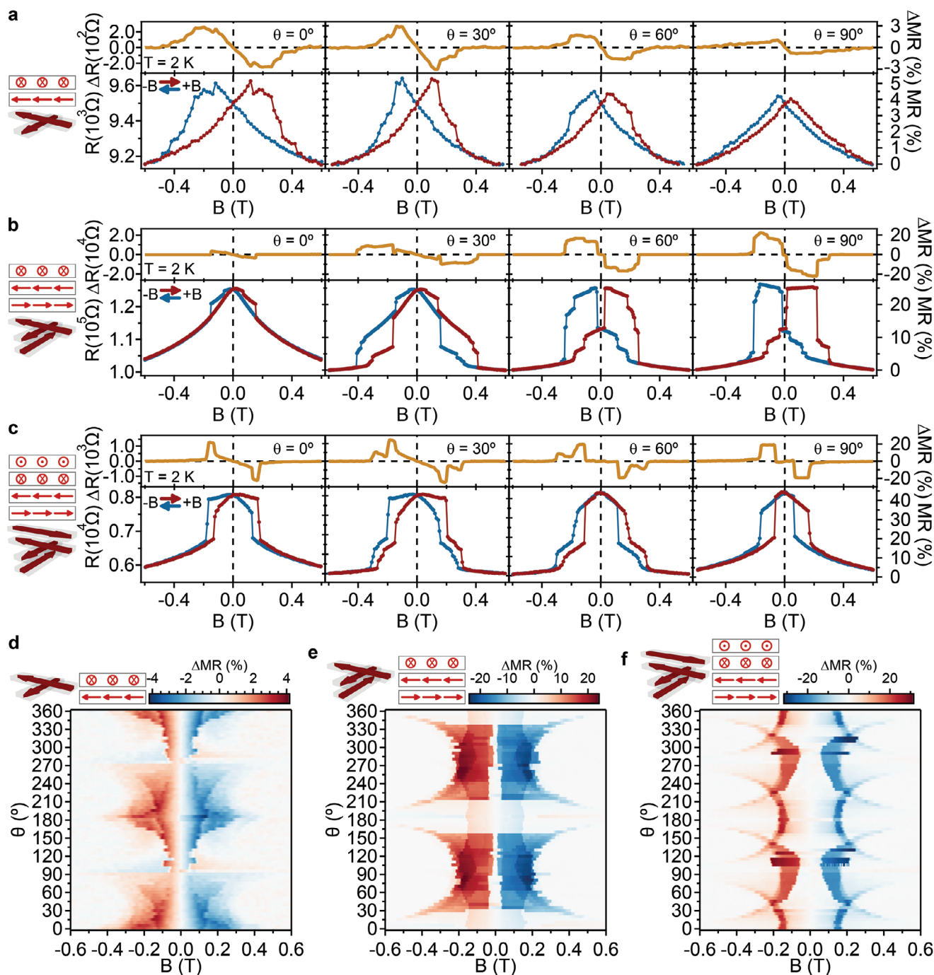
Figure 3. Magnetic switching in orthogonally-twisted CrSB triggered by the field direction. a-c) Magnetic switching at selected angles and d-e) 2D \Delta MR plots for orthogonally-twisted a,d) monolayer/monolayer, b,e) monolayer/bilayer and c,f) bilayer/bilayer CrSB. Sweeping up (down) trace is denoted in red (blue). The full dataset is shown in the Supporting Information Section 1.1.
