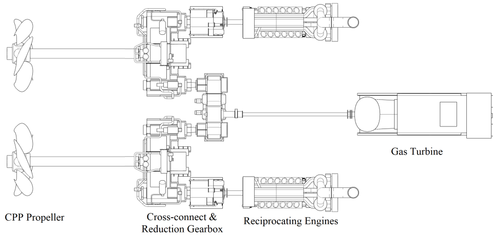
Figure 5: CODOG Propulsion System Layout
