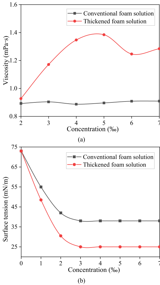
Fig. 19. Comparison of two foam solutions: (a) Viscosity, and (b) Surface tension.
