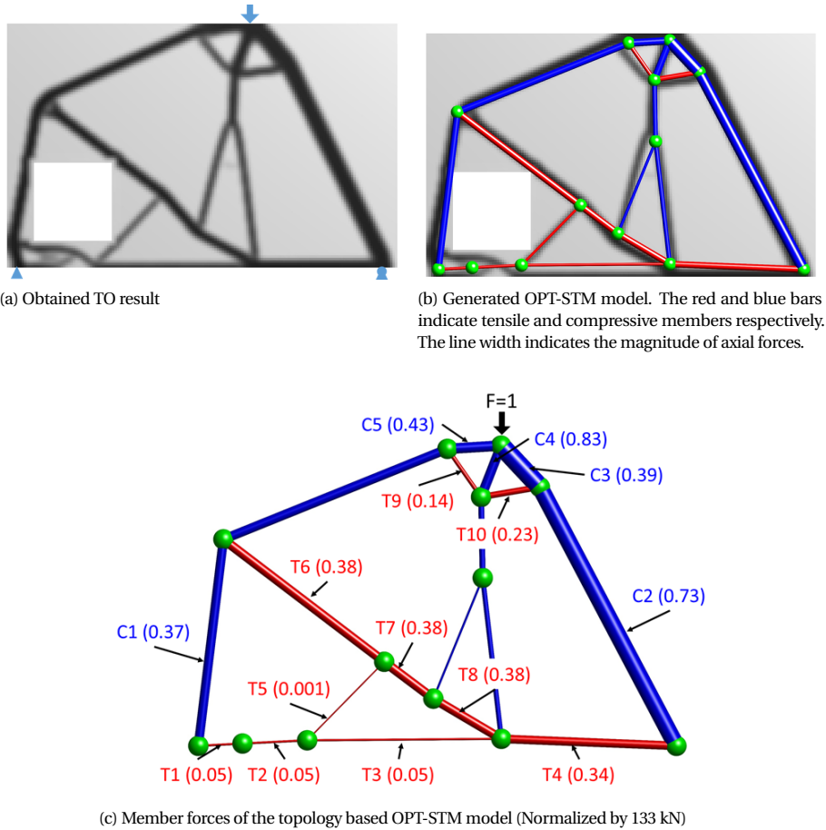
Figure 5.11: OPT-STM results of the deep beam structure
