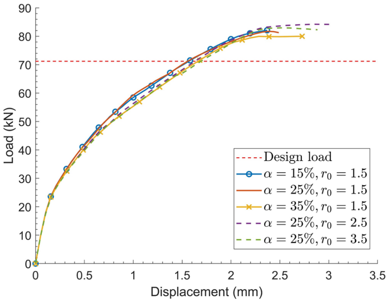
Figure 3.27: Load-displacement curves of evaluated OPT-STM models.
