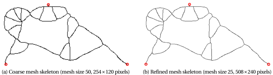
Figure 2.3: Skeletons after the thinning process. The fixed load and boundary points are shown with red circles.
