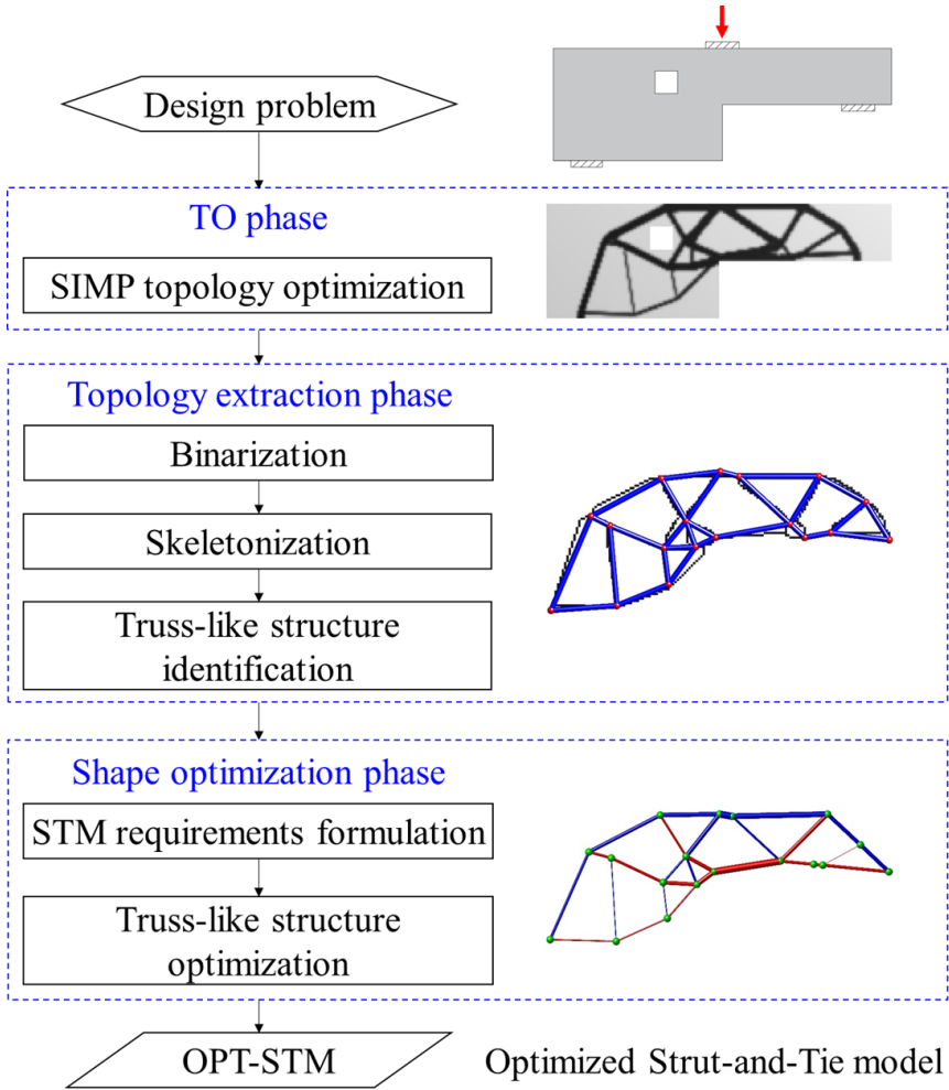
Figure 3.2: Flowchart of the OPT-STM generation method.
