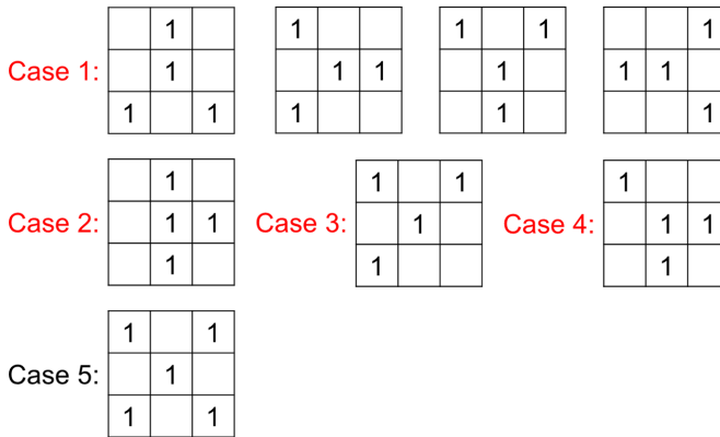
Figure 2.4: Set of patterns used for determining candidate nodes
