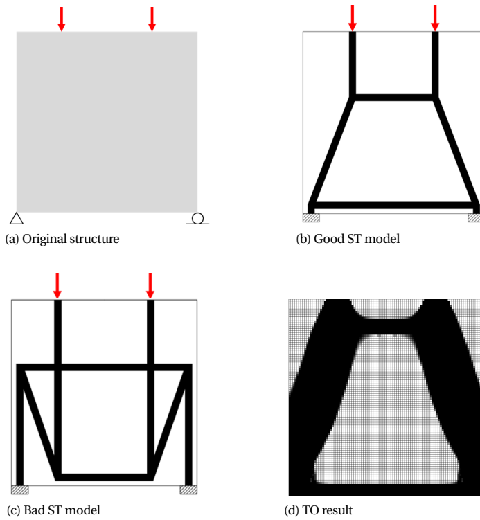
Figure 2.11: Geometries considered to illustrate the evaluation method. (a) shows the deep beam design problem; (b) and (c) show manually generated ST models; (d) shows the TO result.
