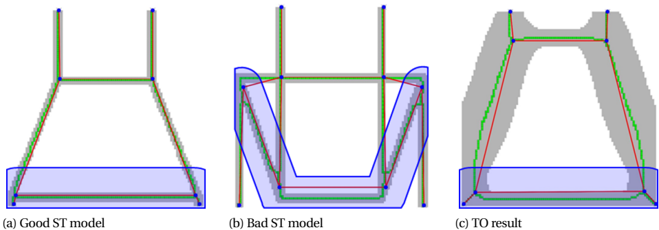
Figure 2.12: Results after image processing and truss extraction. The blue regions indicate the averaging domains in the non-local averaging operation.
