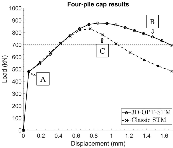
Figure 4.10: Load-displacement results of the 3D-OPT-STM design and classic STM design of the four-pile cap.
