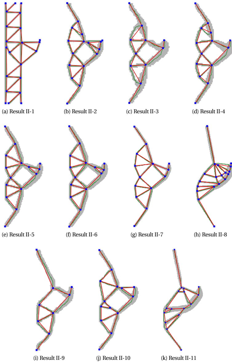
Figure 2.24: Extraction results of Case II: Corbel
