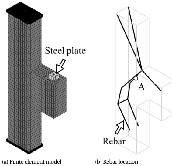
Figure 4.14: NLFEA model of the 3D-OPT-STM design of the corbel. Point A indicates the yielding point of steel.
