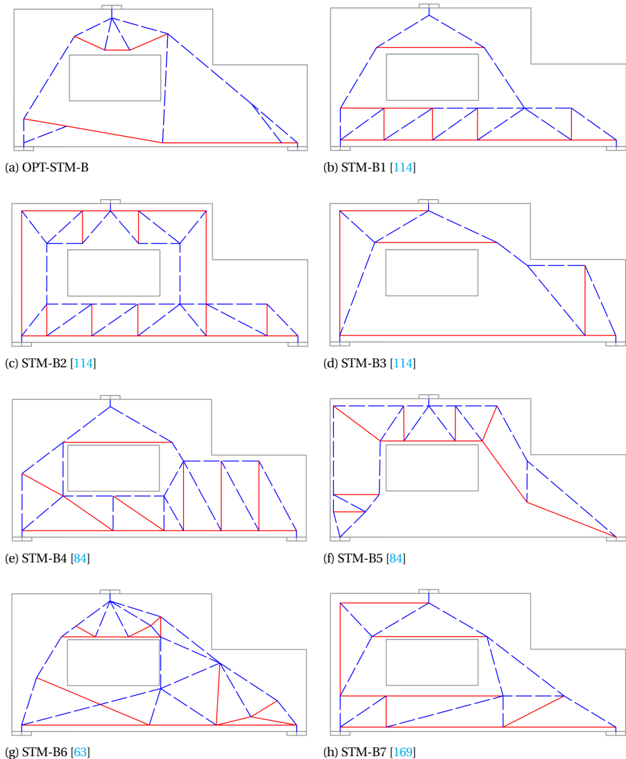
Figure 3.37: ST models for Case B (irregular deep beam).
