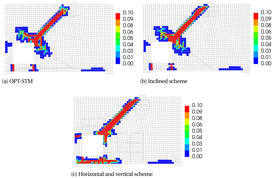
Figure 5.18: The crack patterns at the failure state of three designs (mm)
