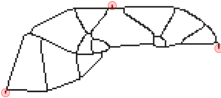
Figure 3.5: The skeleton after the thinning process. The pixels marked in red circles are load and support points, and they are unremovable.
