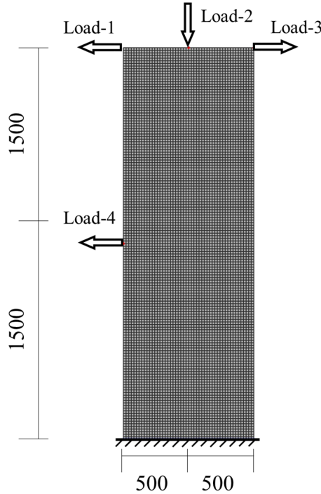
Figure 5.7: Finite element model of the column case (mm)
