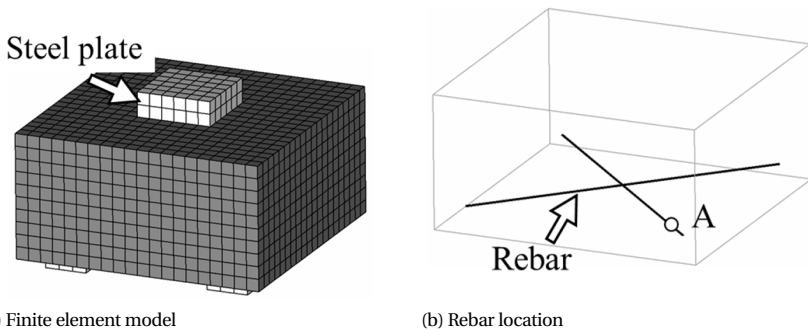
Figure 4.9: NLFEA model of the 3D-OPT-STM design of the four-pile cap. Point A indicates the yielding point of steel.
