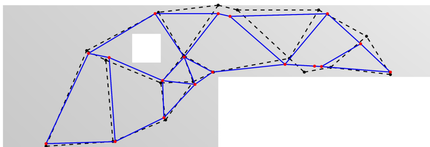
Figure 3.14: Comparison of two models. The blue solid lines present the model after shape optimization, while the black dashed lines present the truss obtained after Step 2.
