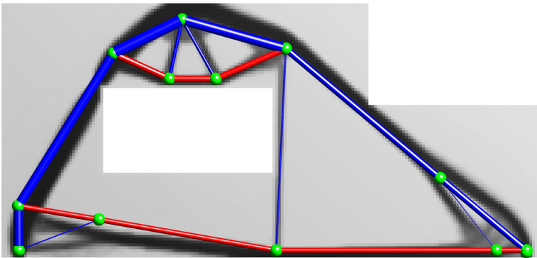
Figure 3.34: The generated OPT-STM of the irregular deep beam.
