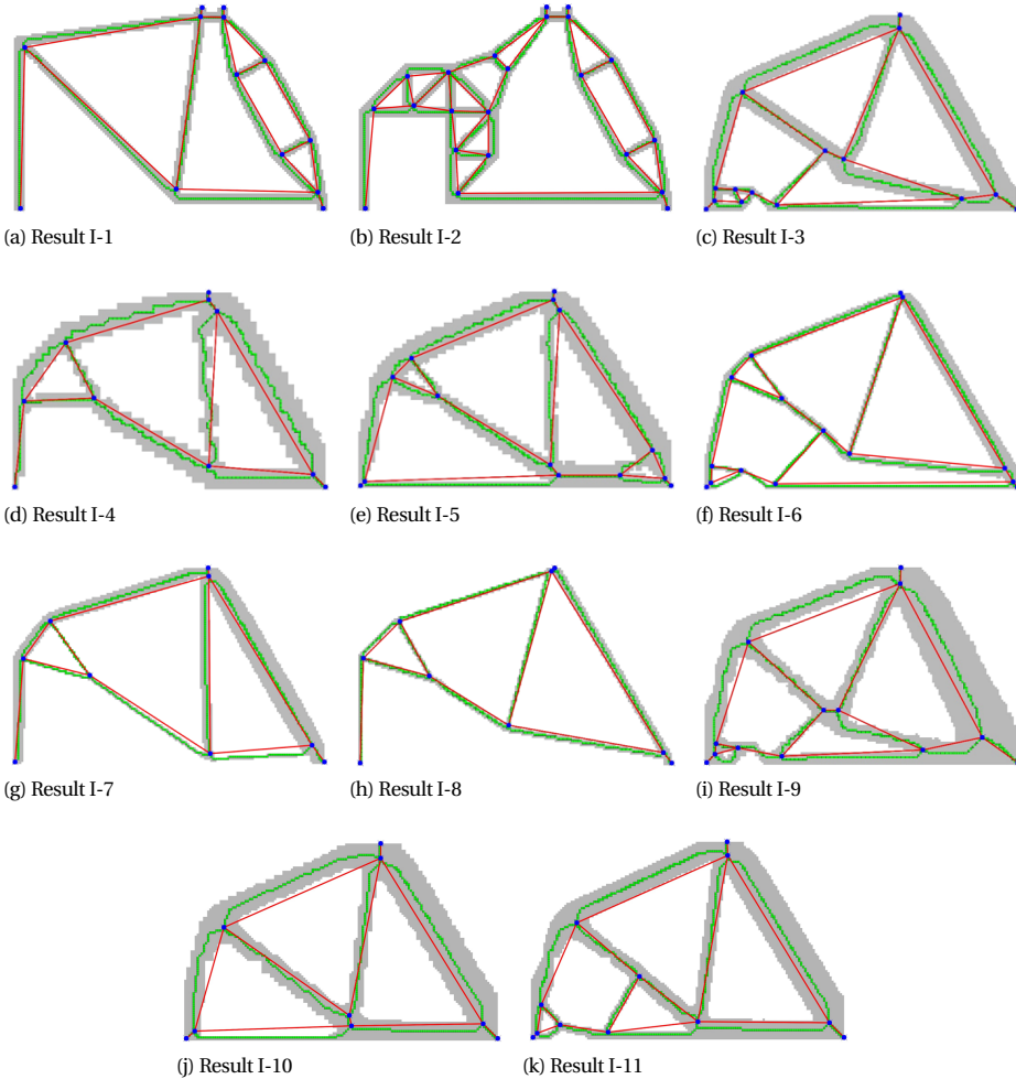
Figure 2.21: Extraction results of Case I: Deep beam with an opening
