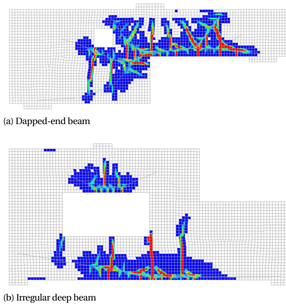
Figure 3.40: Crack plots for the OPT-STM models at the ultimate state.
