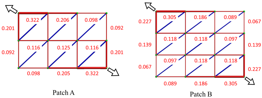
Figure 5.14: Tensile forces of the created grid structure (Normalized by 133 kN). Arrows indicates the force direction from the original inclined ties. The line width indicates the magnitude of axial forces.
