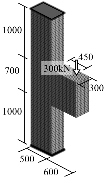
Figure 4.11: The FEM model of the corbel case (mm)
