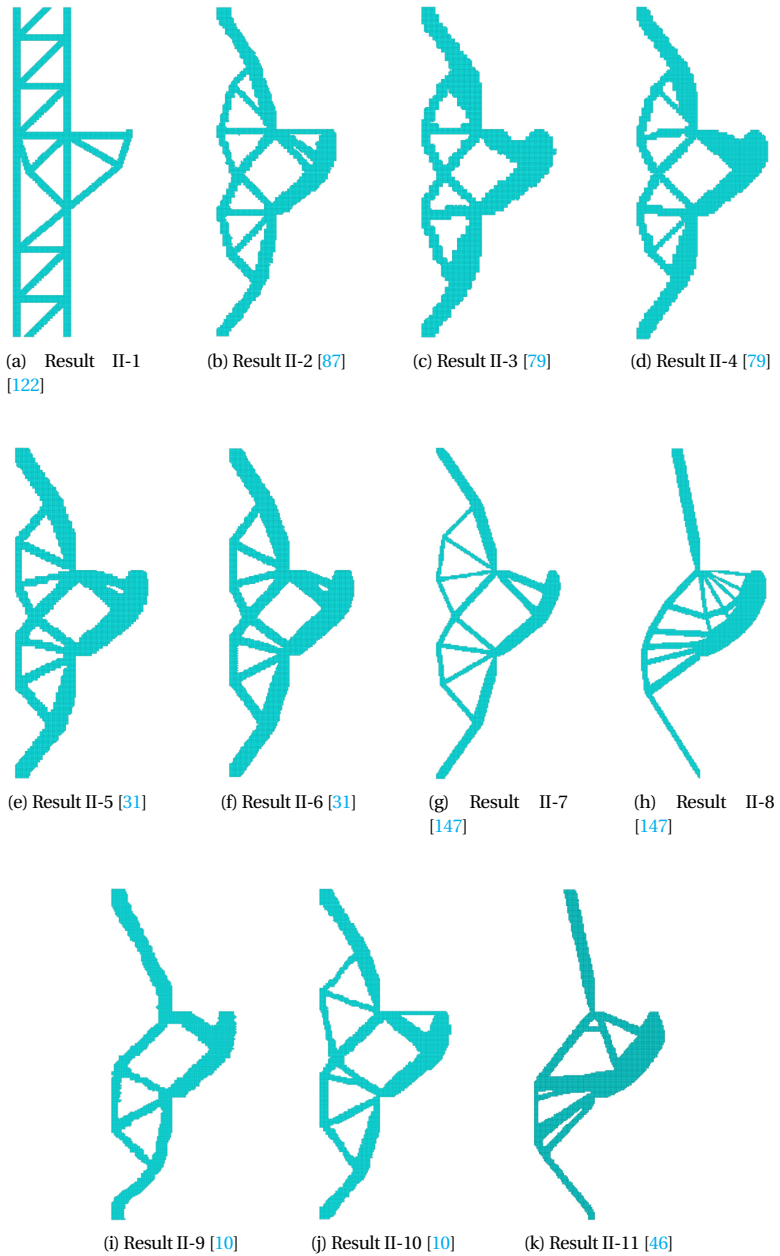
Figure 2.18: Case II: Corbel
