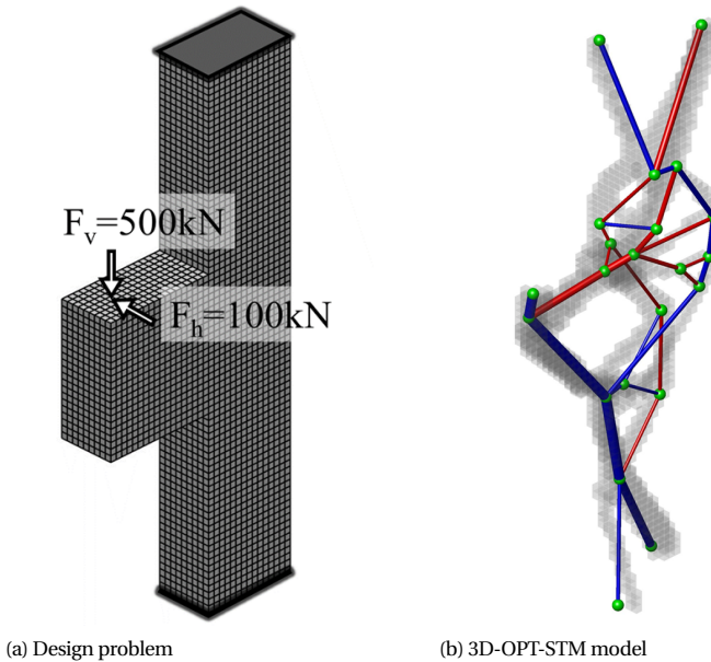
Figure 4.22: The corbel problem under complex load combination. The grey voxels indicate the TO results. Red and blue bars indicate tensile and compressive members respectively. The bar width indicates the force magnitude.
