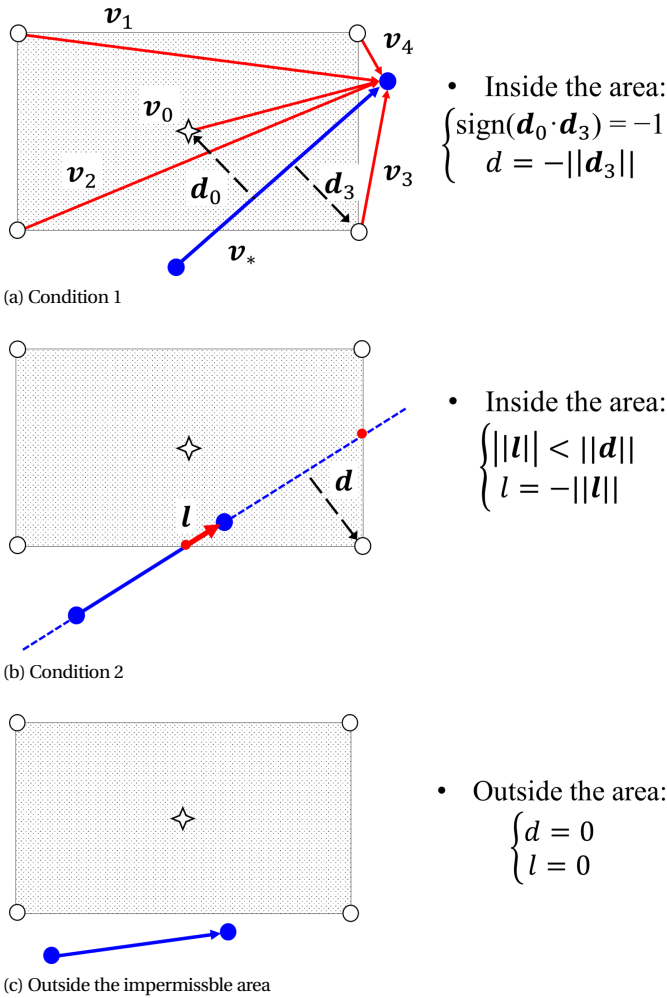
Figure 3.11: Example illustrating the geometry constraint. Blue points indicate two nodes of a bar. Black circles and stars indicate the four corners and the centre point of a rectangular impermissible area respectively. Red points indicate the intersection points.
