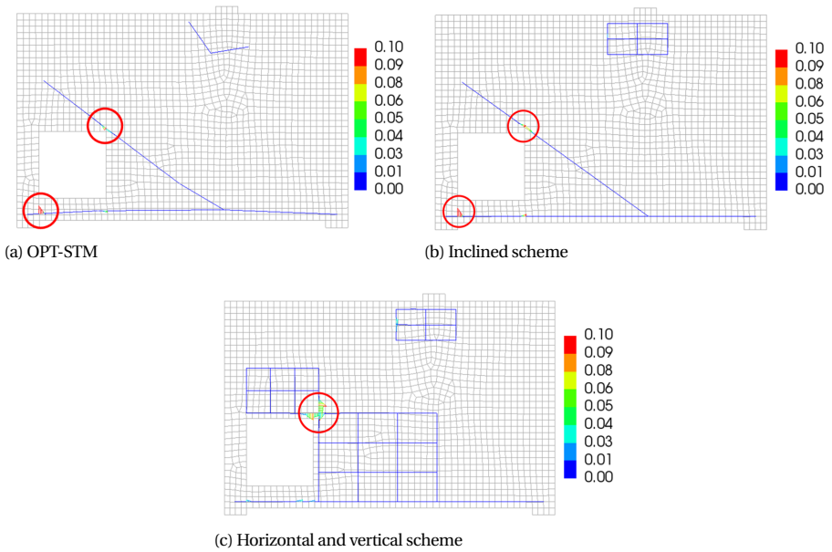
Figure 5.17: The steel strain at the failure state of three designs. Steel rupturing is highlighted with red circles.
