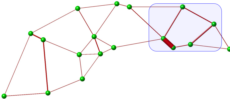
Figure 3.31: The shear force diagram of the uncorrected truss-like structure. The bar width indicates the magnitude of shear forces.
