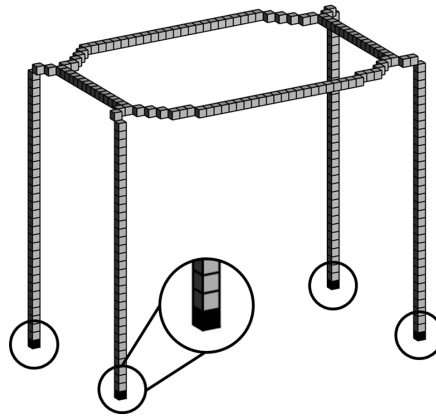
(b) Thinning skeleton (black voxels within circles are the prescribed unremovable members)
