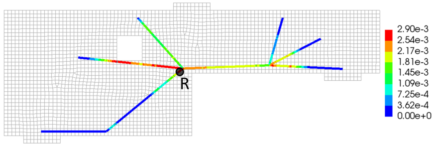
Figure 3.29: Steel strain distribution of the model ( r_L = 25\% ) (Point R indicates the rupturing location).
