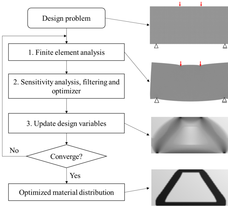
Figure 1.7: Flowchart of the procedures involved in a density-based TO method
