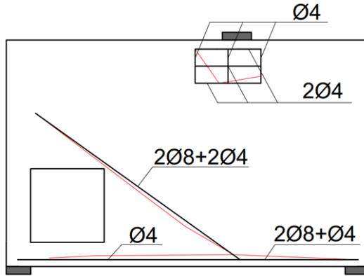
Figure 5.12: The inclined steel design (mm)
