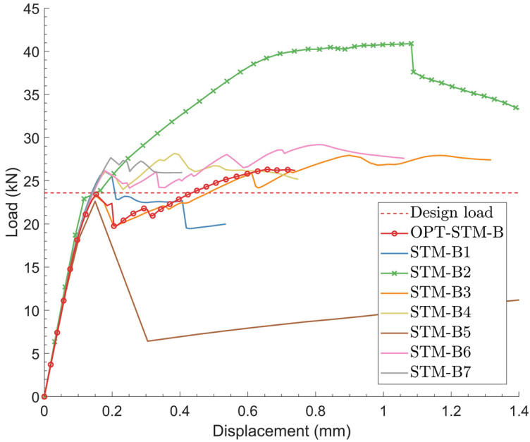
Figure 3.39: The load-displacement curves for the ST models of Case B (irregular deep beam).
