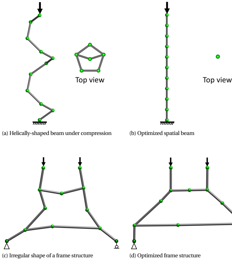
Figure 4.5: Two simple cases and resulting structures after the 3D shape optimization
