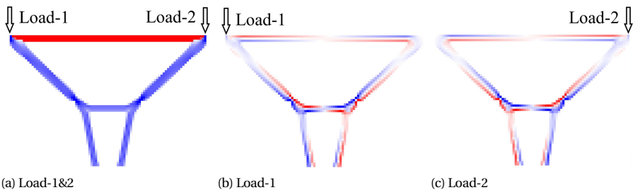
Figure 5.4: Principal stress distribution of the single-load TO result. Red and blue parts indicate the tensile and compressive regions respectively. The intensity of the color indicates the stress magnitude.
