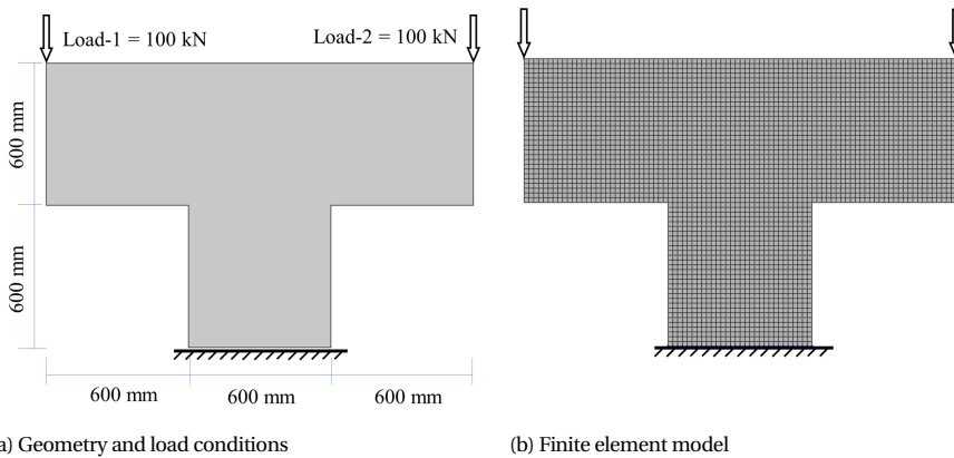
Figure 5.2: Tee joint structure case considering three load combinations, Load-1, Load-2 and Load-1&2.
