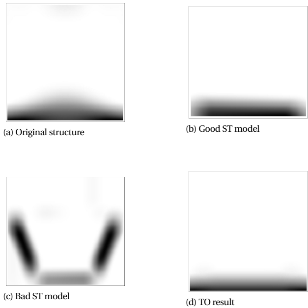
Figure 2.14: Scaled tensile principal stress after non-local averaging
