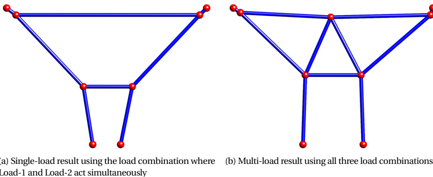
Figure 5.6: Extracted truss-like structures based on the optimized topologies of the tee joint structure
