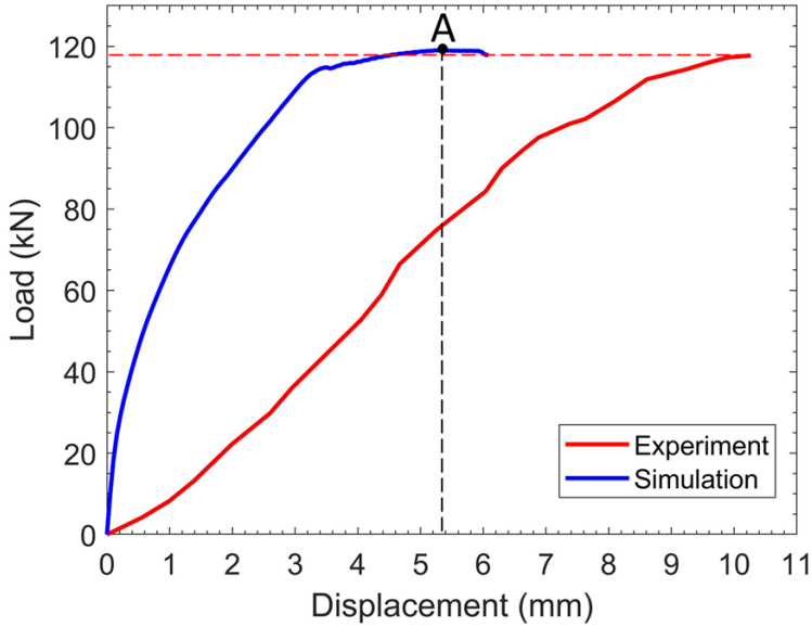
Figure 3.20: Load-displacement curves of the experimentally tested dapped-end beam.
