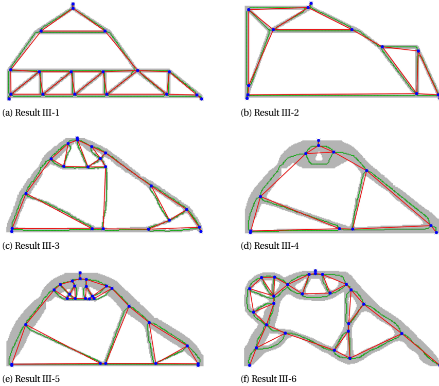
Figure 2.25: Extraction results of Case III: Dapped-end beam with opening
