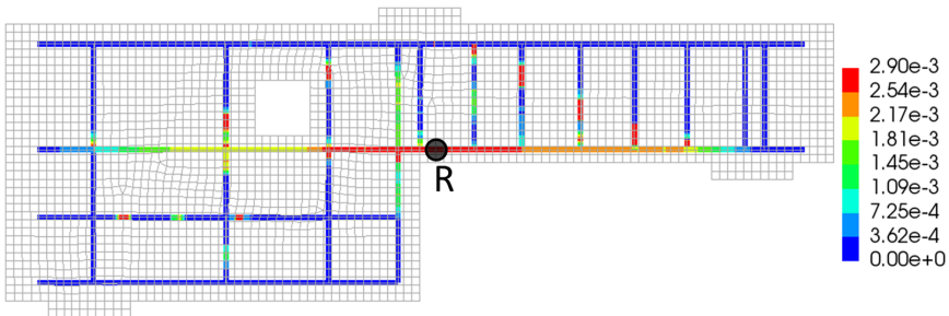
Figure 3.21: Steel strain distribution at the ultimate state B (Point R indicates the rupturing location).
