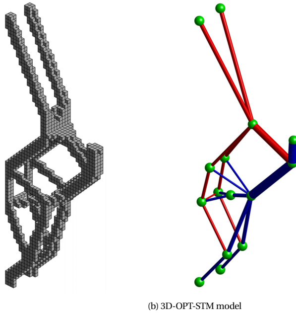
Figure 4.12: Generation results of the corbel case. Red and blue bars indicate tensile and compressive members respectively. The bar width indicates the force magnitude.
