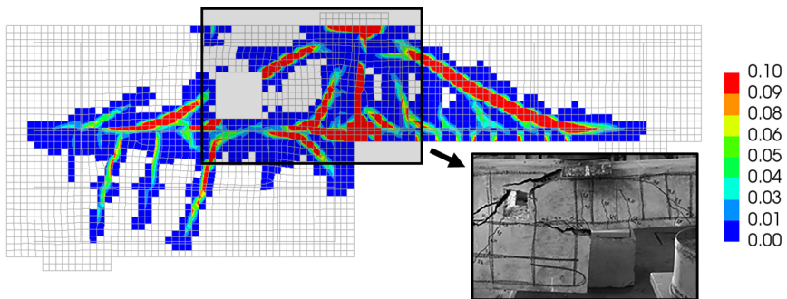
Figure 3.22: Simulated and experimental (inset) crack patterns and widths (mm) at the ultimate state B of the experimentally tested dapped-end beam. The inset is adapted from Oviedo et al. [106].
