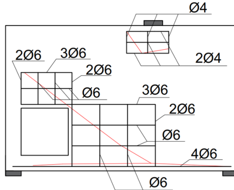
Figure 5.15: The horizontal-and-vertical steel design (mm)
