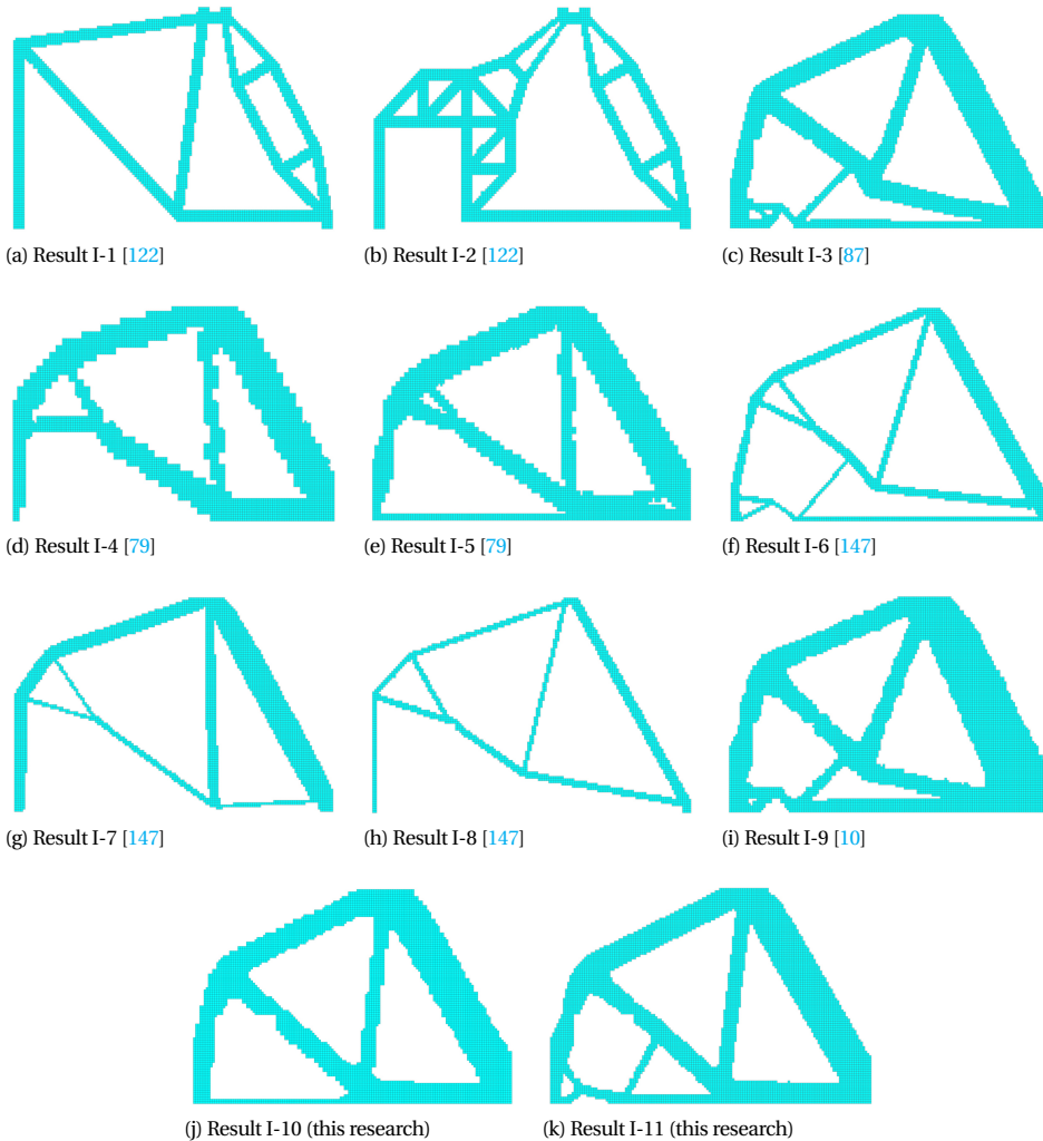
Figure 2.17: Case I: Topology optimized results of the deep beam with an opening
