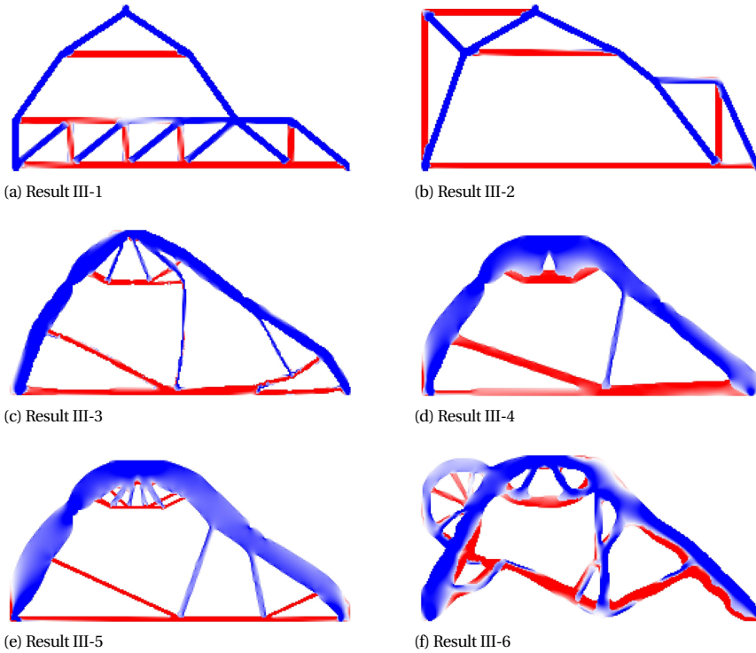
Figure 2.23: Principal stress plots of Case III: Dapped-end beam with opening
