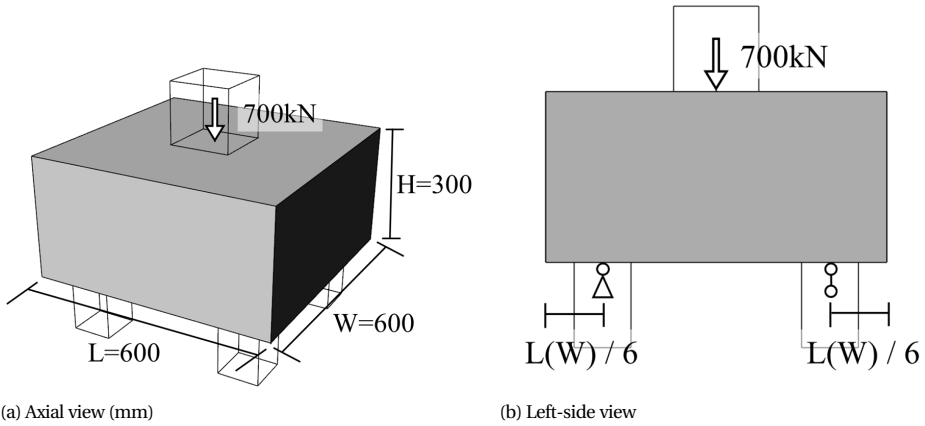
Figure 4.6: Geometry, load and supports of the four-pile cap
