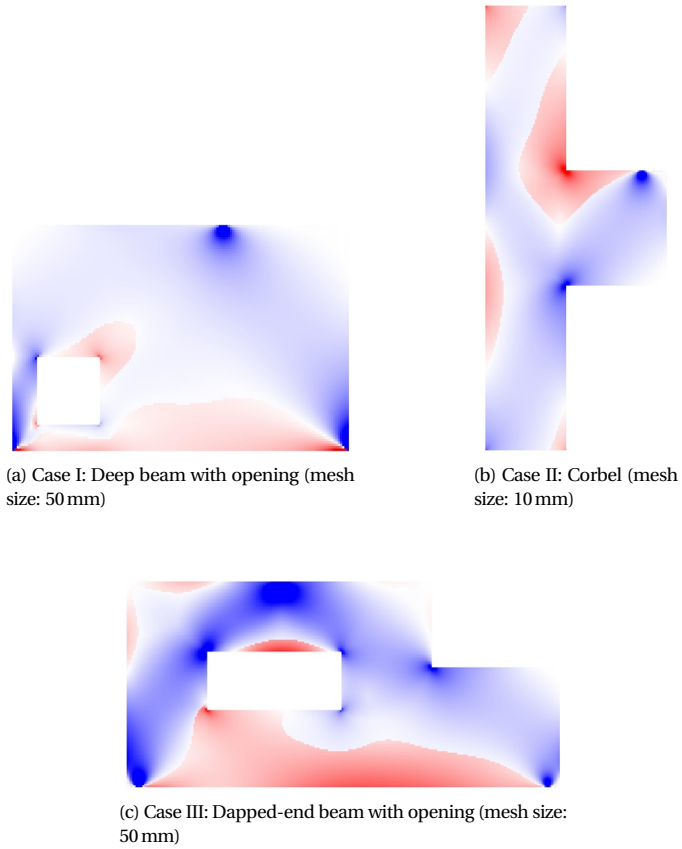
Figure 2.16: Principal stress plots of three cases. Red and blue parts indicate the tensile and compressive regions respectively.
