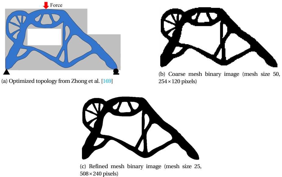
Figure 2.2: Generating binary designs based on a TO result
