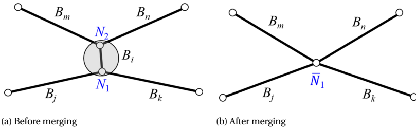
Figure 3.9: The example of merging a short bar.
