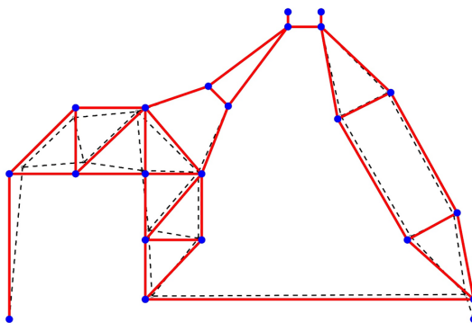
Figure 2.27: Truss-like structure of Result I-2. Dashed lines indicate the generated truss-like structures and solid lines show the adjusted structure.
