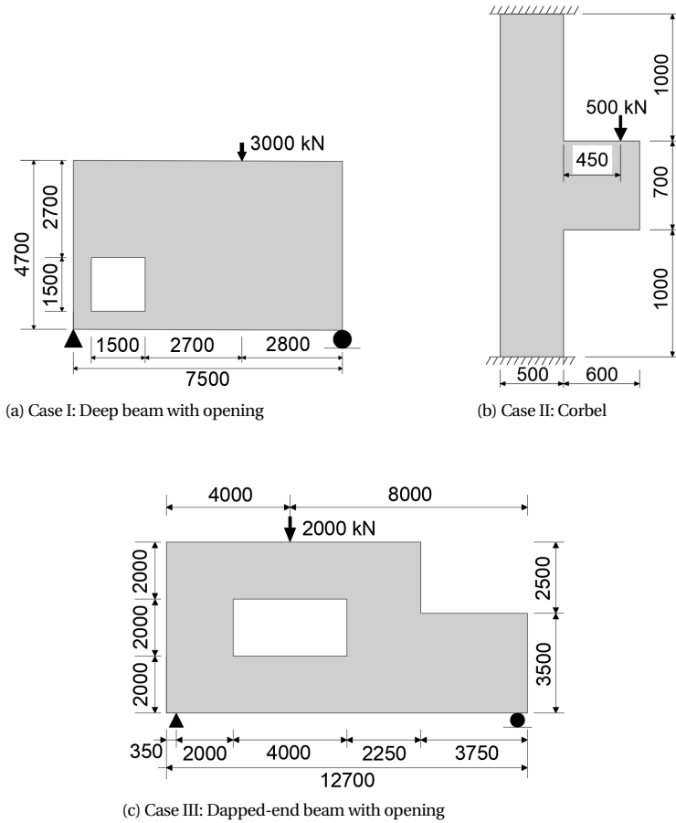
Figure 2.15: Basic information of three cases (mm)
