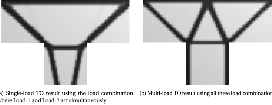
Figure 5.3: Optimization results of the tee joint structure with respect to two TO formulations
