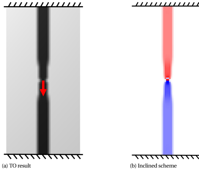
Figure 6.1: Illustrative example of a column constrained at both sides with an axial load at its center. Red and blue parts indicate tensile and compressive stress. The intensity of the color indicates the stress magnitude. Standard TO leads to equal forces in the strut and tie, in absolute sense. A more economical solution would be obtained by only using a strut.
