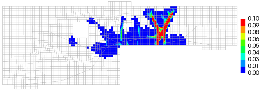
(a) Simulated crack patterns and widths (mm)
