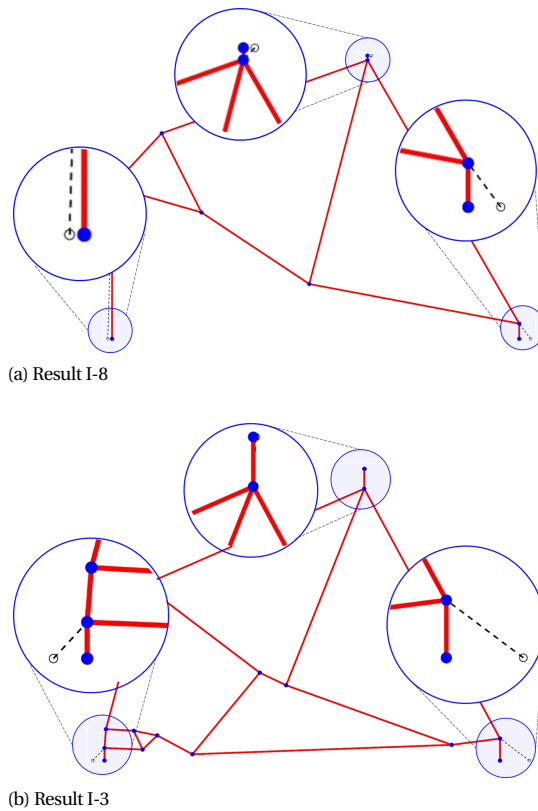
Figure 2.28: Truss-like structure with zoomed-in details. Dashed lines indicate the generated truss-like structures and solid lines show the adjusted structure.
