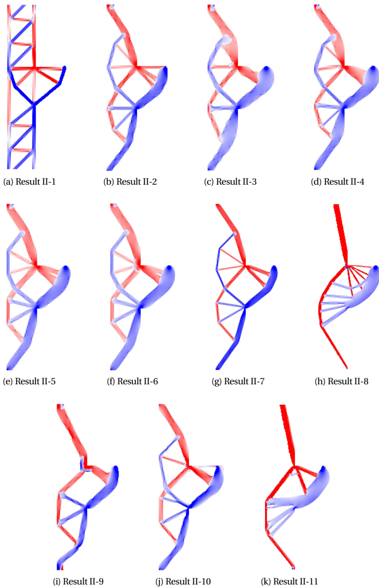
Figure 2.22: Principal stress plots of Case II: Corbel
