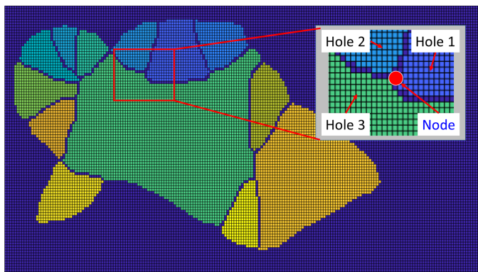
Figure 2.7: Identification of holes and topology relation of a node
