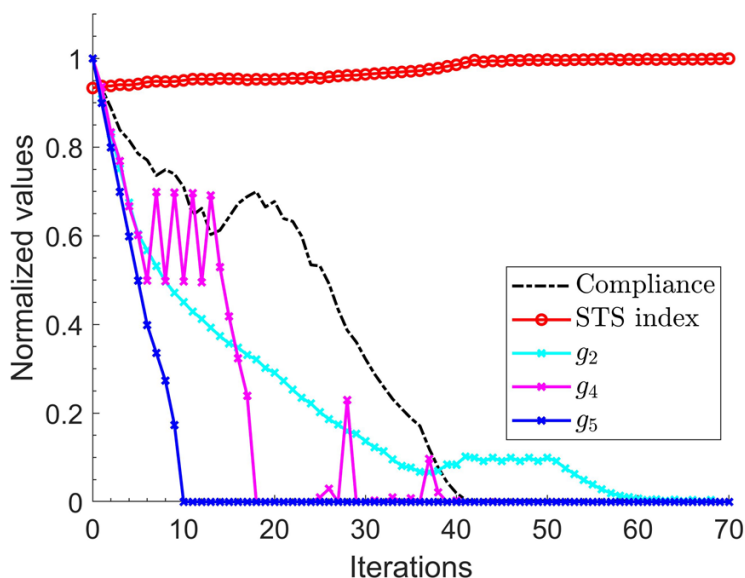
Figure 3.15: Shape optimization convergence history.
