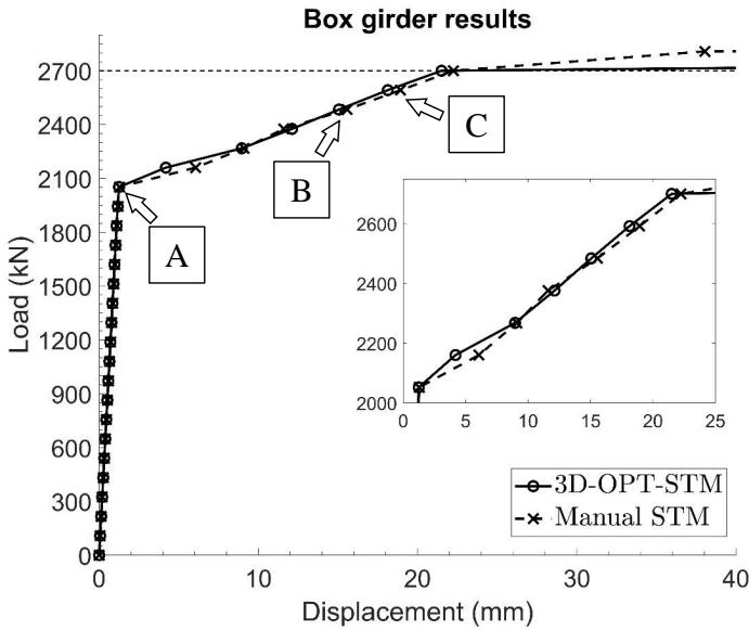
Figure 4.20: Load-displacement results of the 3D-OPT-STM design and classic STM design of the box girder.
