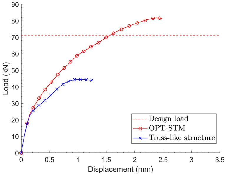
Figure 3.30: Load-displacement curves of the OPT-STM and the uncorrected truss-like model.
