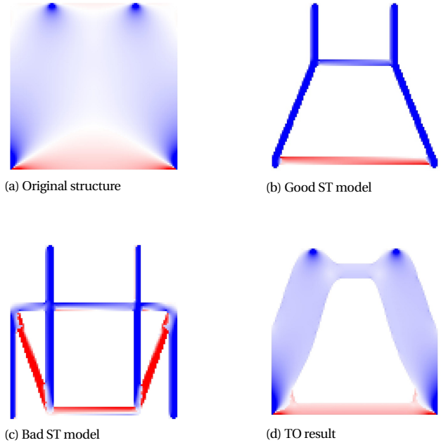
Figure 2.13: Principal stress plots. Red and blue parts indicate the tensile and compressive regions respectively.
