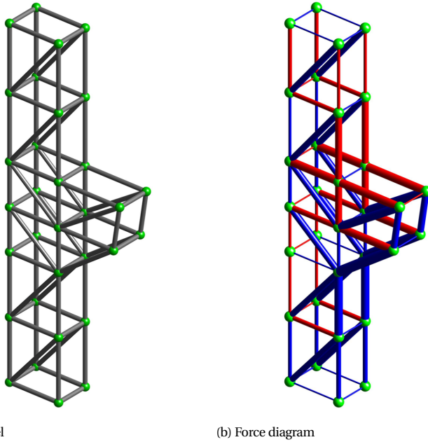
Figure 4.13: The manually created ST model of the corbel. Red and blue bars indicate tensile and compressive members respectively. The bar width indicates the force magnitude.
