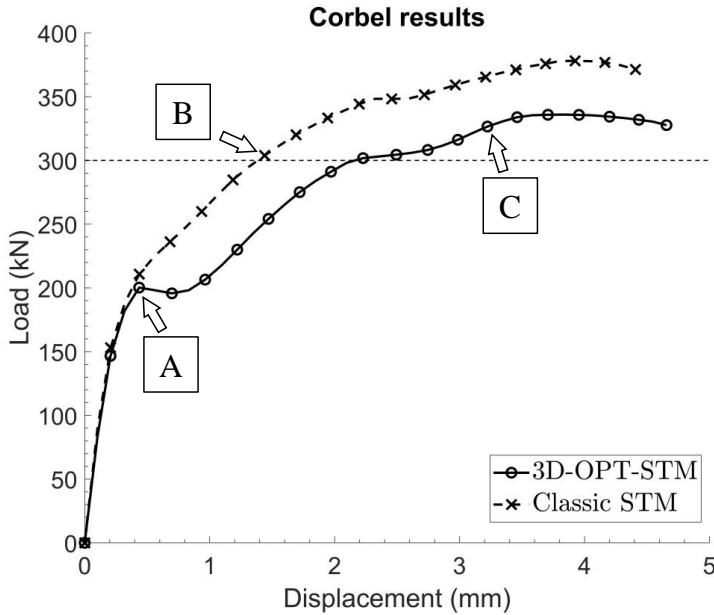
Figure 4.15: Load-displacement results of the 3D-OPT-STM design and classic STM design of the corbel.
