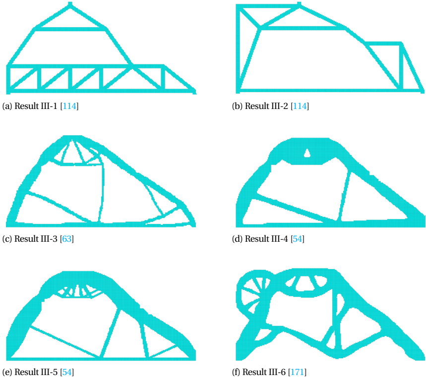
Figure 2.19: Case III: Dapped-end beam with opening
