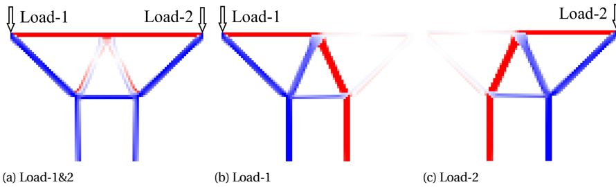
Figure 5.5: Principal stress distribution of the multi-load TO result. Red and blue parts indicate the tensile and compressive regions respectively. The intensity of the color indicates the stress magnitude.
