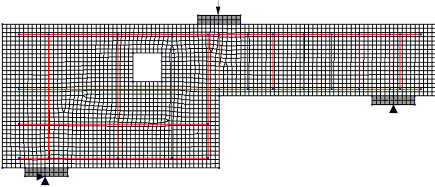
Figure 3.19: Finite element model of the experimentally tested dapped-end beam.
