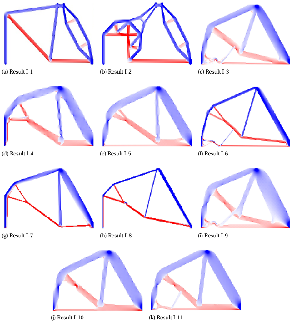
Figure 2.20: Principal stress plots of Case I: Deep beam with an opening. Red and blue parts indicate the tensile and compressive regions respectively
