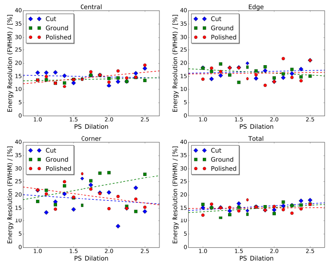
Fig. 7. Energy resolution (FWHM) for four LYSO array crystal region classifications: 1) central (top left); 2) edge (top right); 3) corner (bottom left); and 4) total (bottom right). The colored dashed lines correspond to a fitted linear function for each crystal surface type to illustrate the general trend as a function of PSI.
