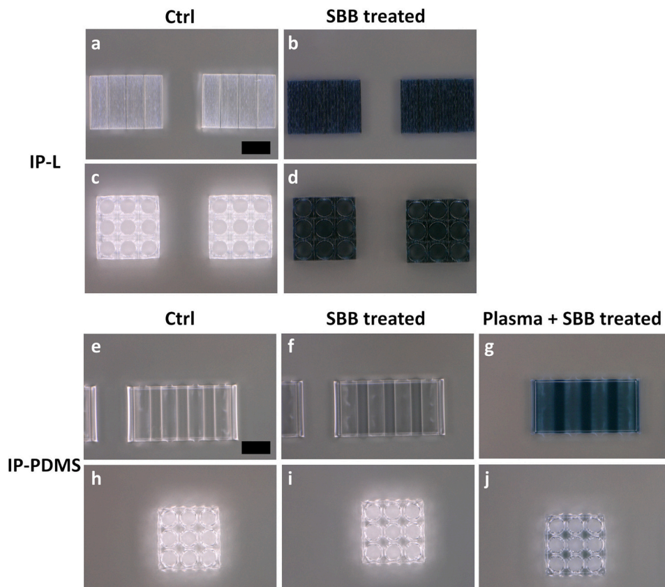
Fig. 3. Optical microscope images of (a,c) untreated IP-L fabricated structures (i.e. controls), (b,d) SBB treated IP-L structures, (e,h) untreated IP-PDMS fabricated structures, (f,i) SBB treated IP-PDMS fabricated structures, (g,j) IP-PDMS structures pre-treated with oxygen plasma for 30 s and then treated with SBB. Scale bar = 50 μm.
