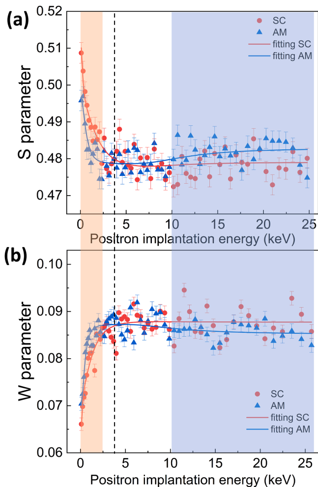
Fig. 5. (a) S parameter and (b) W parameter as a function of the positron implantation energy extracted from positron Doppler broadening (DB) depth profiles for the AM (blue) and the SC (red) sample.
