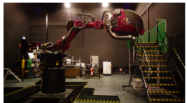
Figure 1: The CyberMotion Simulator (CMS) at the Max Planck Institute for Biological Cybernetics.
