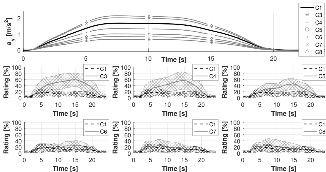
Figure 2: Lateral specific force presented in each condition (top), and average ratings given for all conditions. Shaded areas indicate the mean rating plus/minus one standard deviation. Condition C1 corresponds to k_y = 1.0 , C3 to k_y = 0.4 , C4 to k_y = 0.5 , C5 to k_y = 0.6 , C6 to k_y = 0.8 , C7 to k_y = 1.2 and C8 to k_y = 1.275 .
