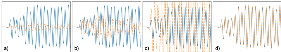
Figure 4.9: Plots with surface-related multiples as found in the data (solid blue line) and the repredicted surface-related multiples (dashed orange line). The Green's function used for reprediction is: a) the result of R-EPSI, b) the result of R-EPSI multiplied by k_z , c) the result of R-EPSI multiplied with \sqrt{i\omega} , d) the result of R-EPSI multiplied by \sqrt{i\omega} and a scaling factor of 0.396.
