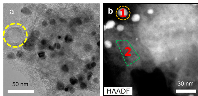
Figure 4. (a) TEM pictures of Co@NC-800 ( al ), (b) HAADF image of Co@NC-800 ( al ).
