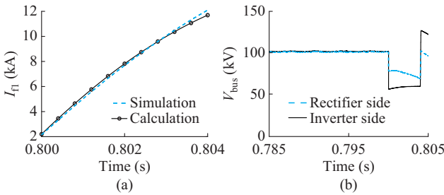
Fig. 13. Fault current and DC bus voltage without SP-PFC. (a) Simulation and calculation results of fault current. (b) Simulation results of DC bus voltage at rectifier and inverter sides.
