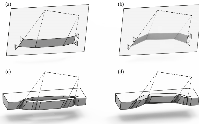
Figure 5.6: The proposed spatial bi-stable unit. (a-b) Two stable states of a conceptual bi-stable unit. They are mirror images of each other against the mirror defined by the four anchors. (c-d) Two stable states of the corresponding physically manufacturable bi-stable unit. The dashed lines are the extension of the hinges. They intersect at points defining the dash-dotted line which serves as the virtual rotation axis of the center piece.
