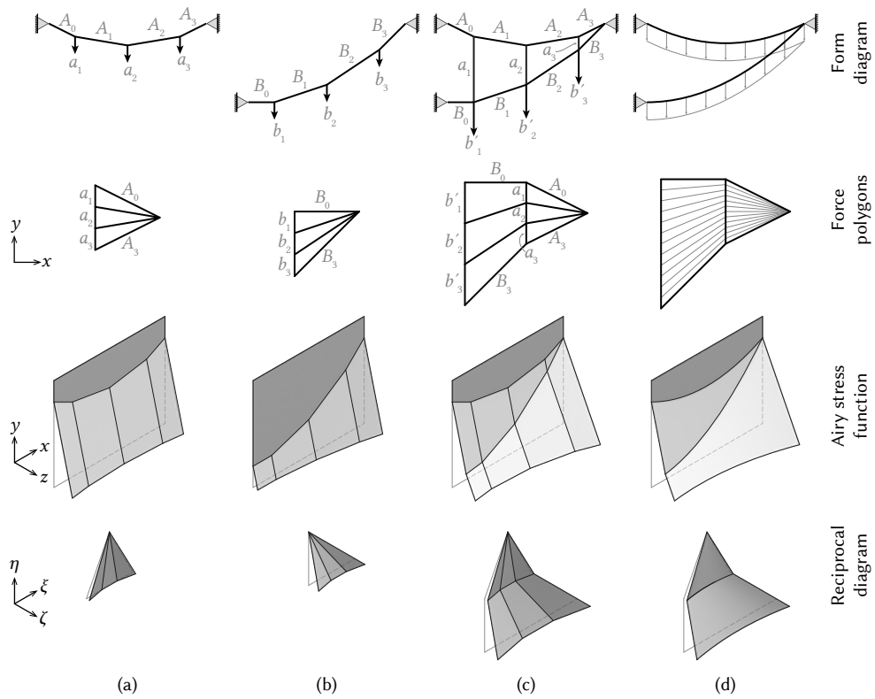
Figure 4.12: Hanging-chain models with corresponding force polygons and Airy stress functions. (a) A chain supporting three weights and anchored at leveled supports. (b) Another chain anchored at differing heights. (c) Two hanging chains in the same vertical plane. (d) Two chains with evenly distributed loads.
