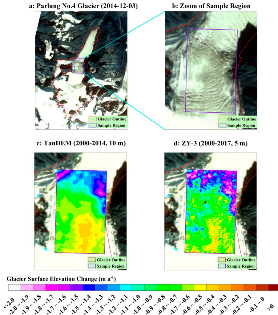
Figure 15. The detail comparison of glacier elevation change derived by TanDEM-X and ZY-3 TLA data for the Parlung No.4 glacier. (a): overview of the Parlung No.4 glacier (the basemap is the 8 m spatial resolution Gaofen-1 true color image with band 4 (R), band 3 (G) and band 2 (B) composition on 3 December, 2014); (b): zoom figure of the sample region; (c) and (d): the annual glacier elevation change derived by TanDEM-X in 2000–2014 and ZY-3 TLA data in 2000–2017; their spatial resolutions are 10 m and 5 m, respectively.
