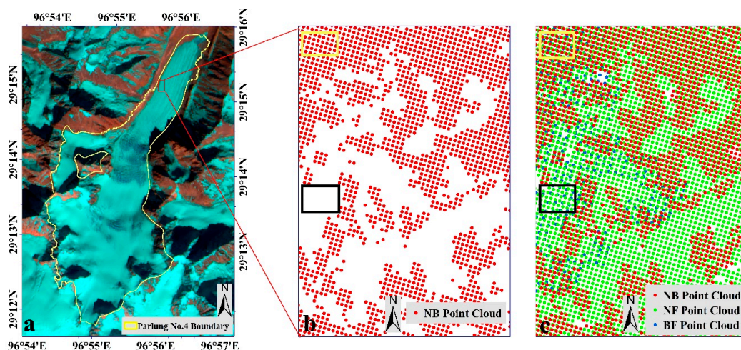
Figure 6. The point cloud of the Parlung No.4 glacier derived by ZY-3 TLA data. (a) The overview of the Parlung No.4 glacier (The basemap is the same as in Figure 1b); (b) The point cloud generated with the one pair (NB) combination; (c) The point cloud obtained by fusing the NB (red points), NF (green points) and BF (blue points) observations.
