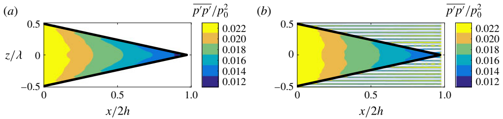
FIGURE 17. (Colour online) Intensity of the mean surface pressure fluctuation \overline{p'p'}/p_0^2 : (a) sawtooth and (b) combed-sawtooth serration. The serration edge in the x-z plane is indicated by means of continuous black lines.
