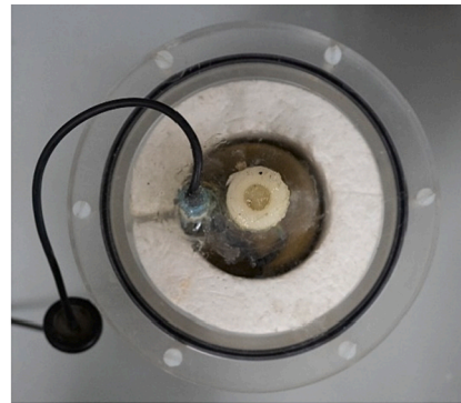
Fig. 3. Calorimetric unit of JAF60 isothermal calorimeter.
