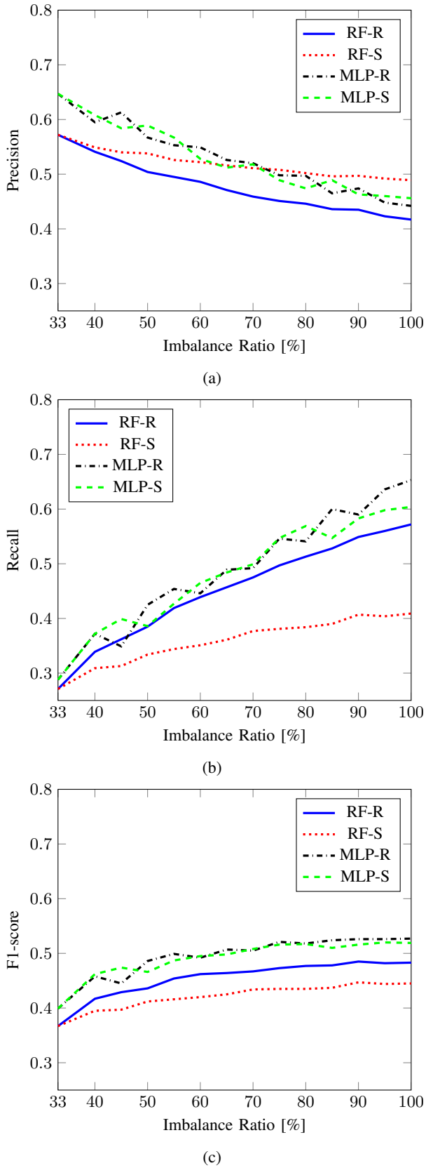
Fig. 5: Precision (a), recall (b) and F1-score (c) as function of the imbalance ratio, for arrival delay prediction (RF = Random Forest, MLP = Multilayer Perceptron, R = RUS, S = SMOTE).
