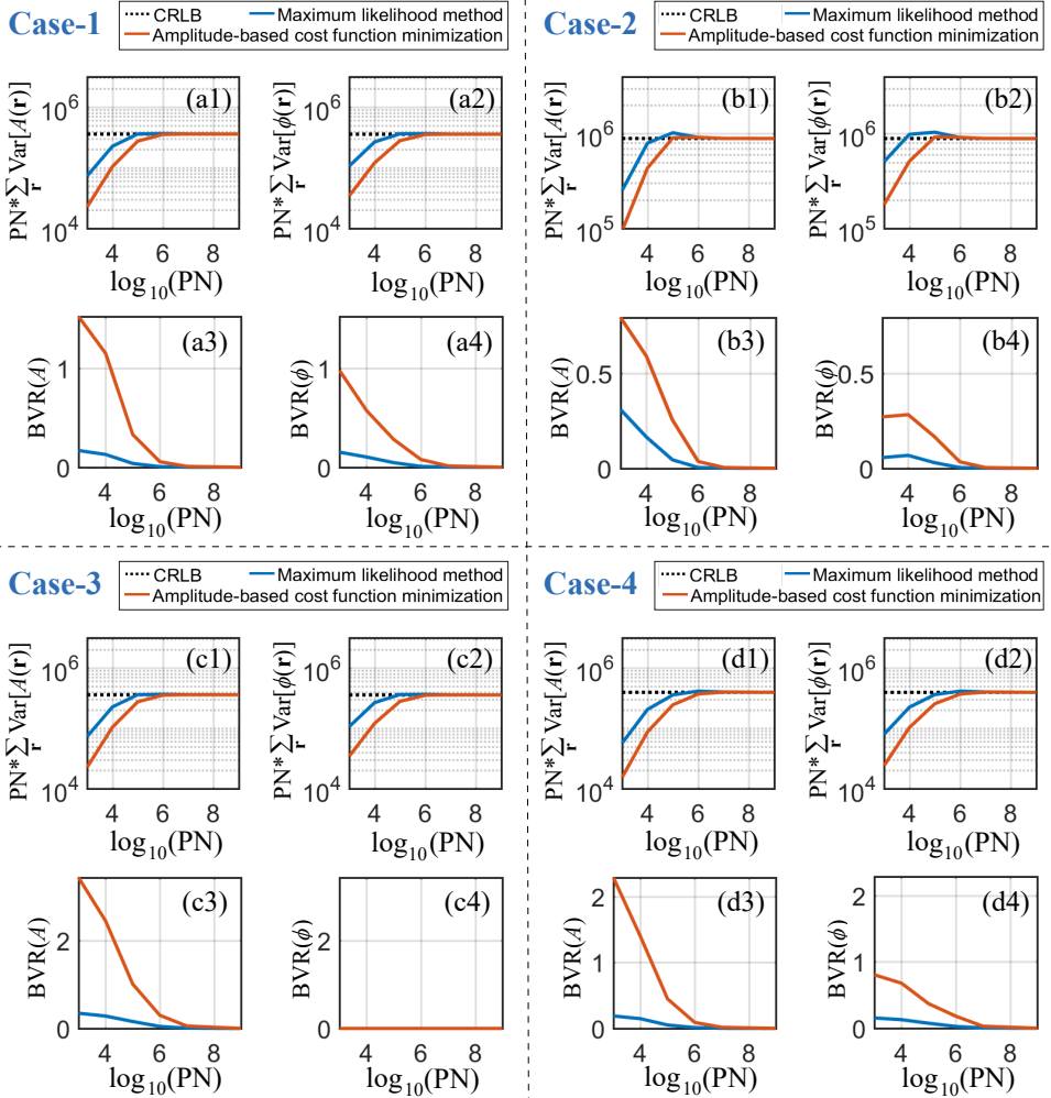
Figure 3.9: The CRLB, variance and bias-variance-ratio of two algorithms for various values of PN. The value of BVR( \phi ) in (c4) is much smaller than BVR(A) in (c3), which agree with the Monte Carlo result shown in Fig. 3.7b and Fig. 3.7d.
