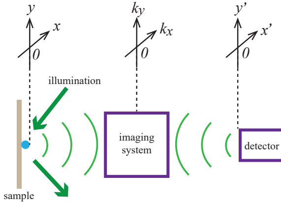
Figure 4.2: Illustration of the setup of application 1. The incident angle of the illumination is 60 degree, with multiple azimuth incident directions around 360 degree.
